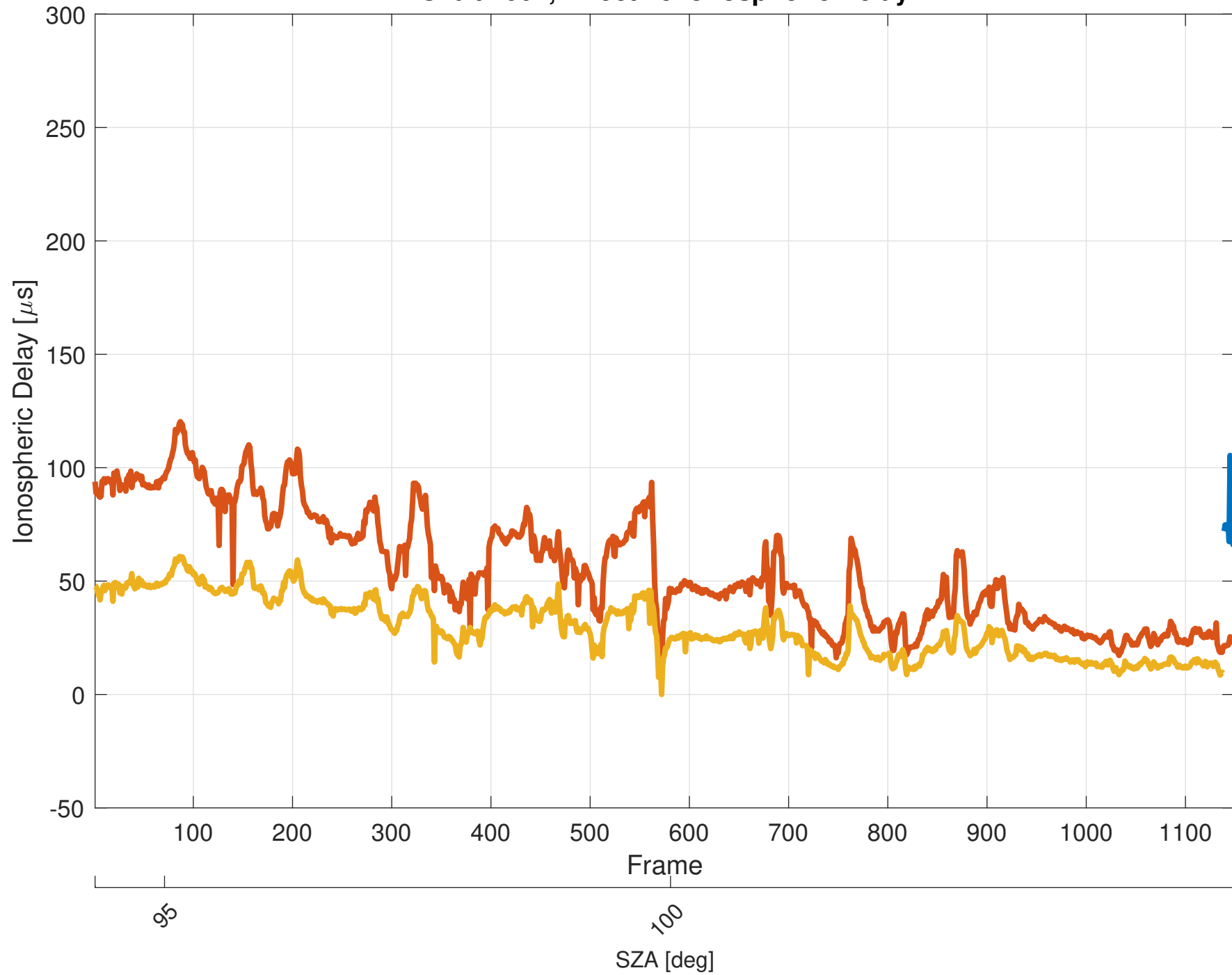
Orbit 4002, Effective Ionospheric Delay
