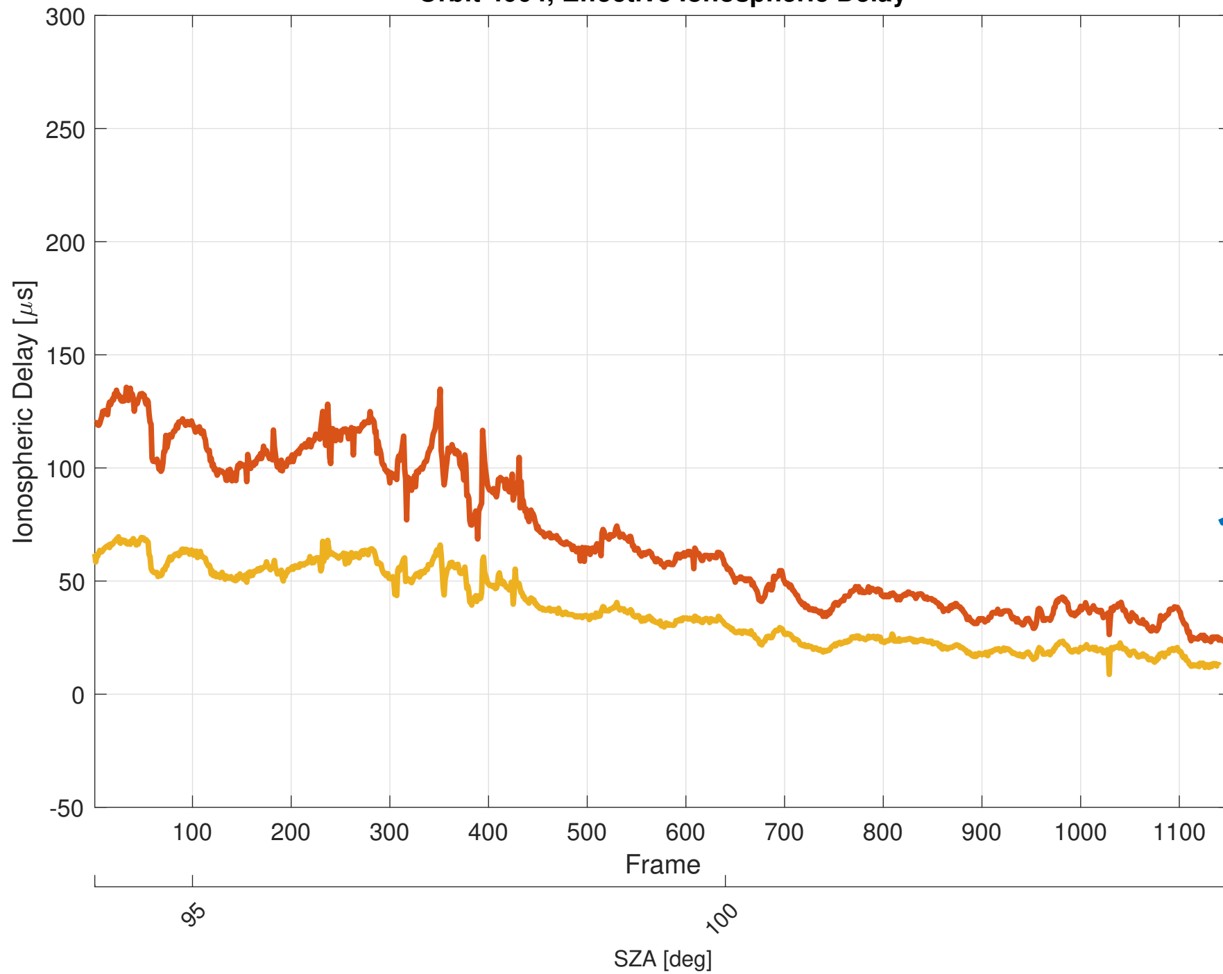
Orbit 4004, Effective Ionospheric Delay
