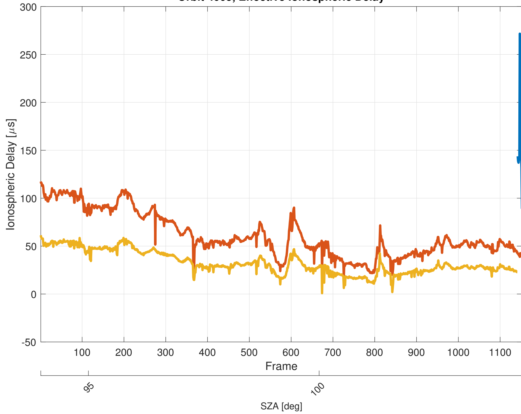
Orbit 4005, Effective Ionospheric Delay
