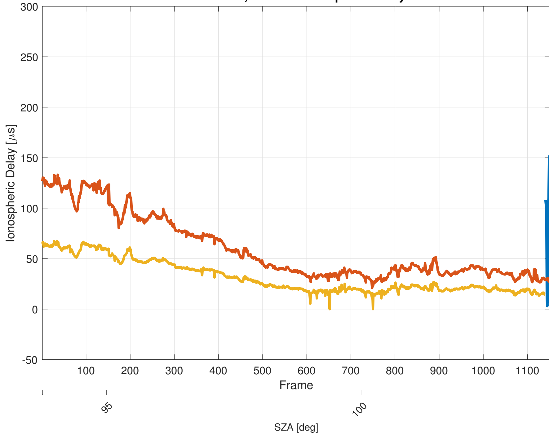
Orbit 4007, Effective Ionospheric Delay
