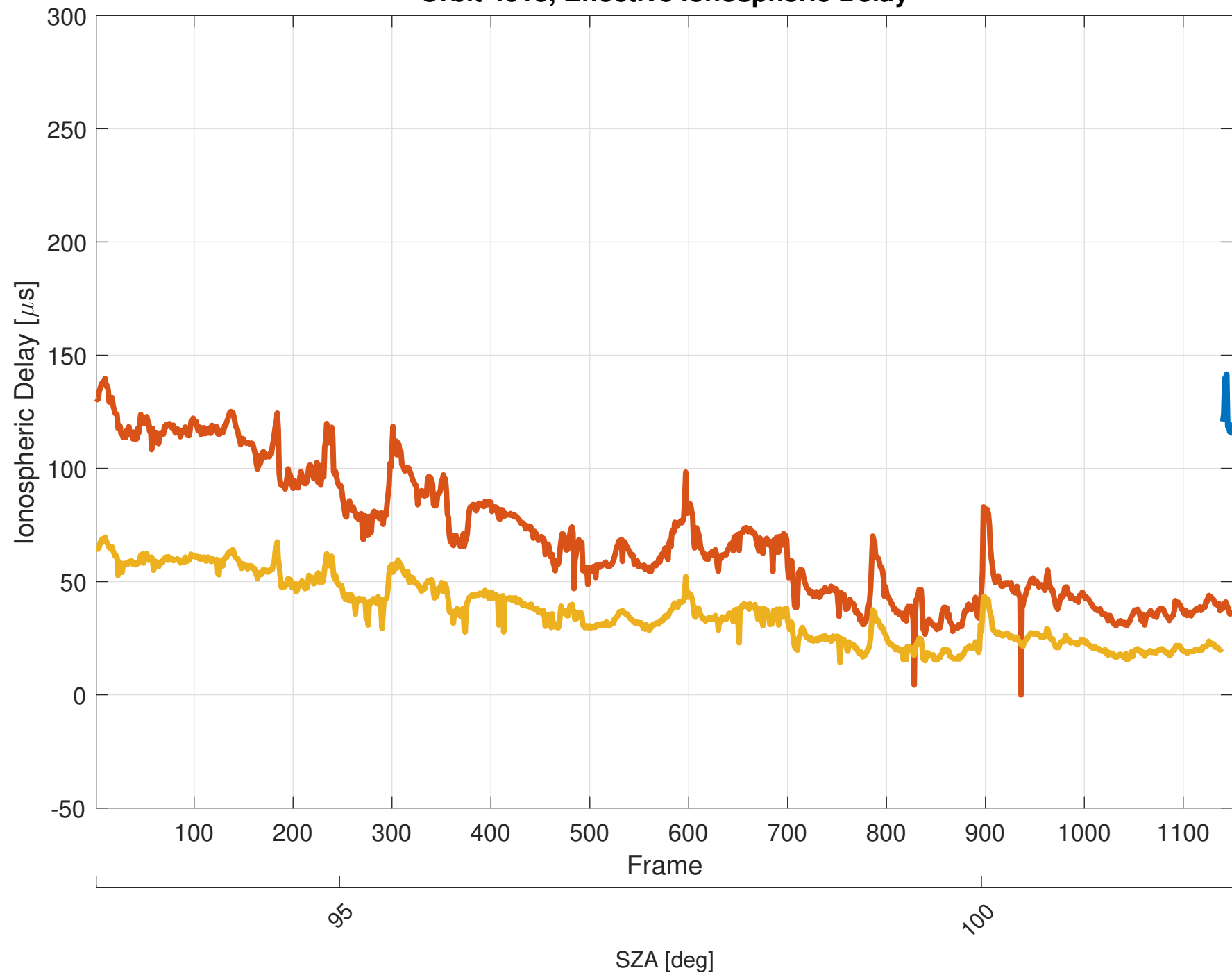
Orbit 4013, Effective Ionospheric Delay
