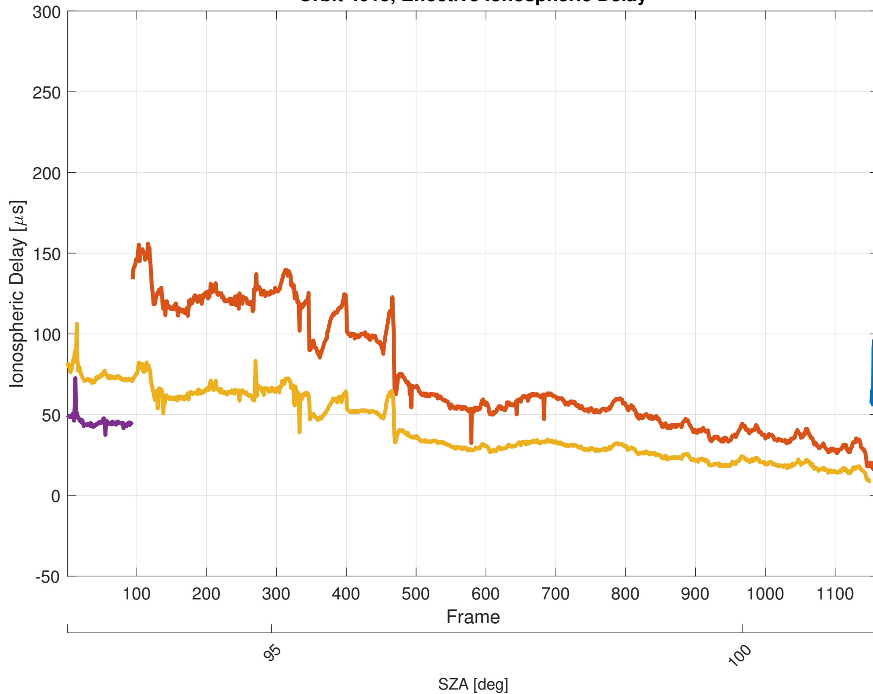
Orbit 4015, Effective Ionospheric Delay
