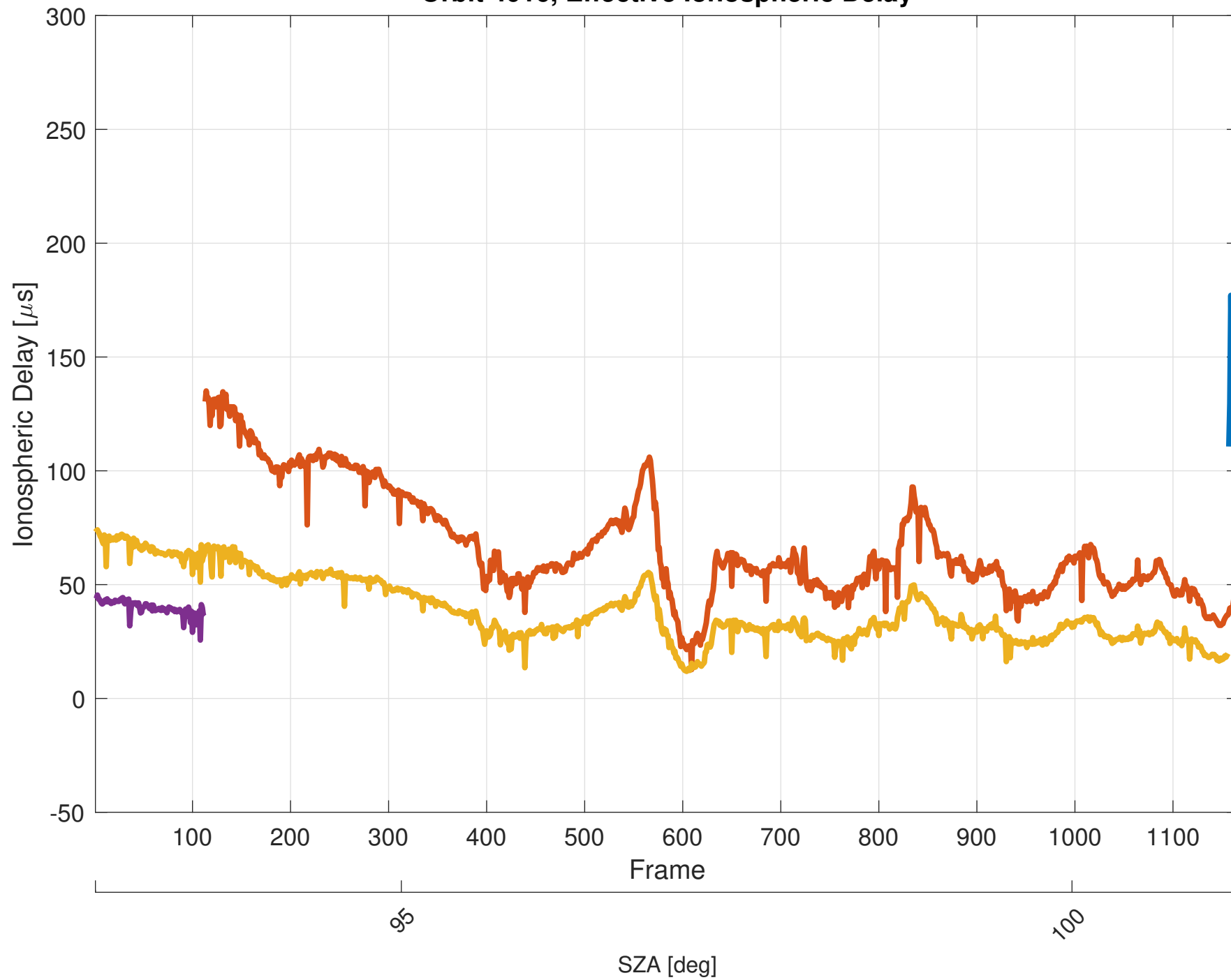
Orbit 4016, Effective Ionospheric Delay
