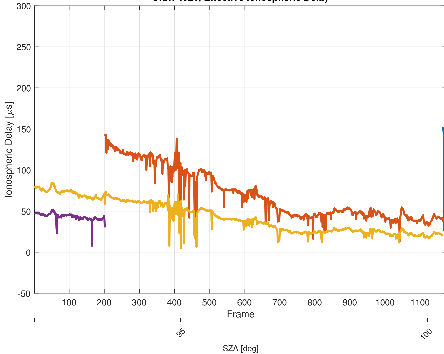
Orbit 4021, Effective Ionospheric Delay
