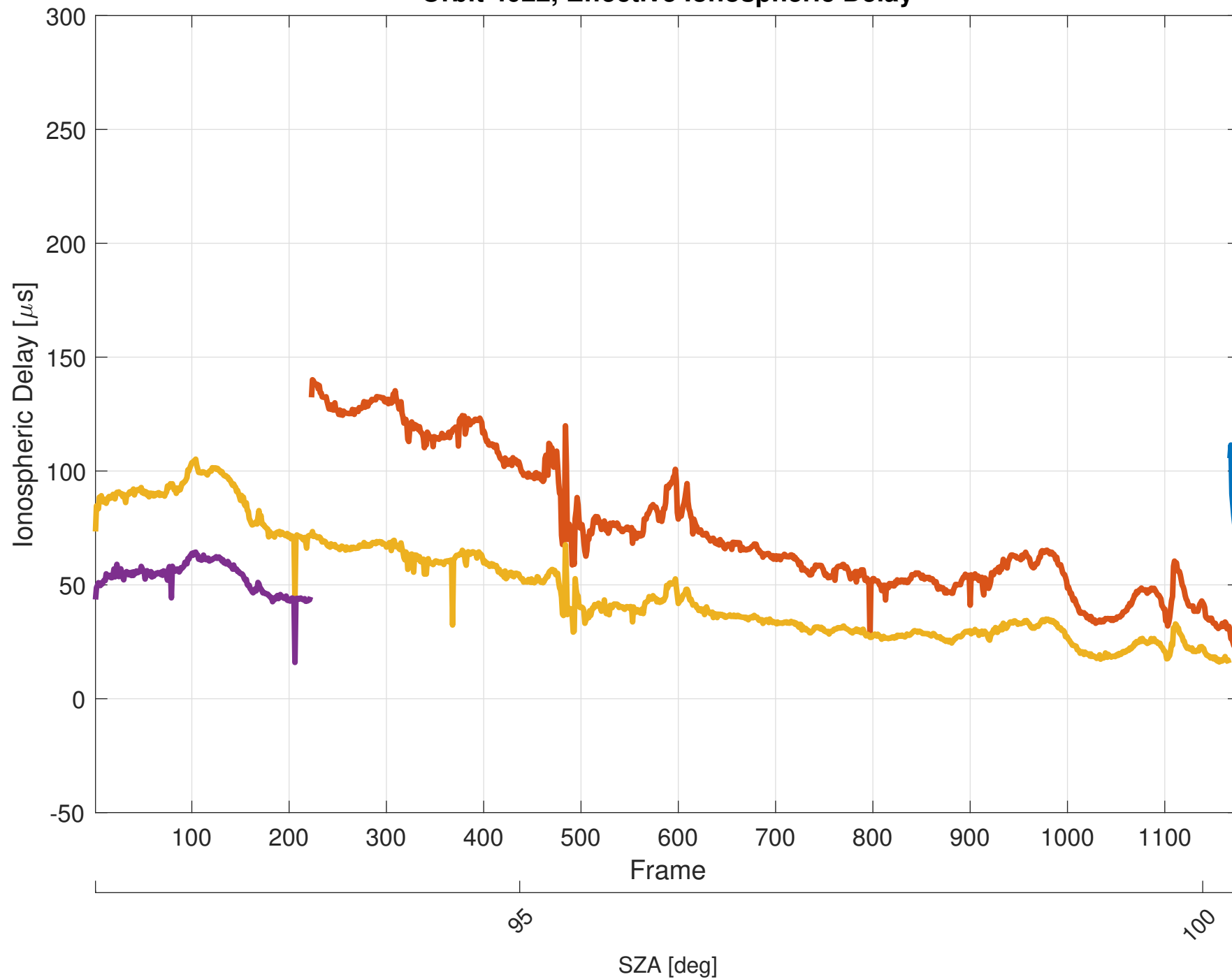
Orbit 4022, Effective Ionospheric Delay
