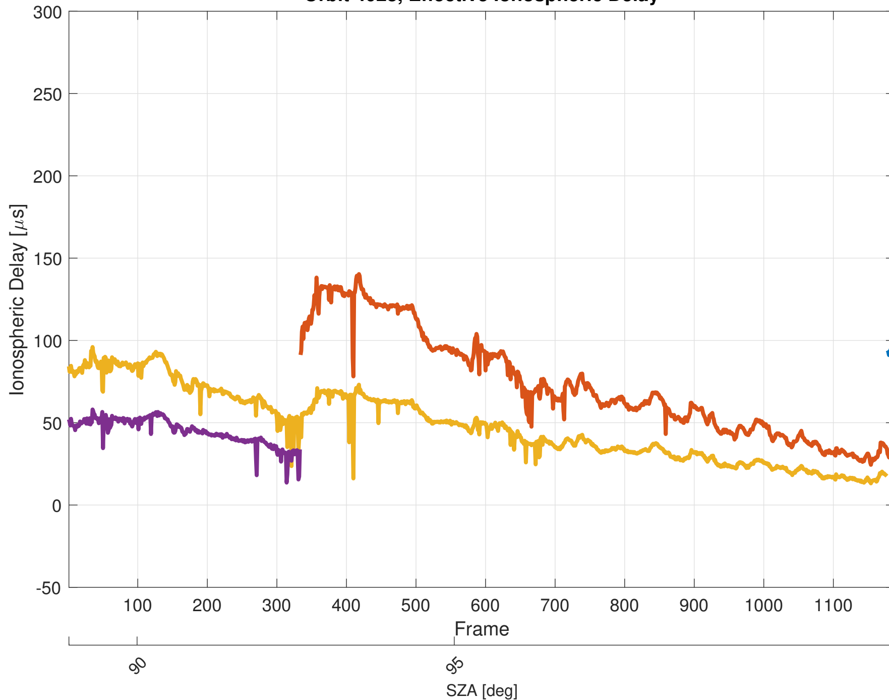
Orbit 4028, Effective Ionospheric Delay
