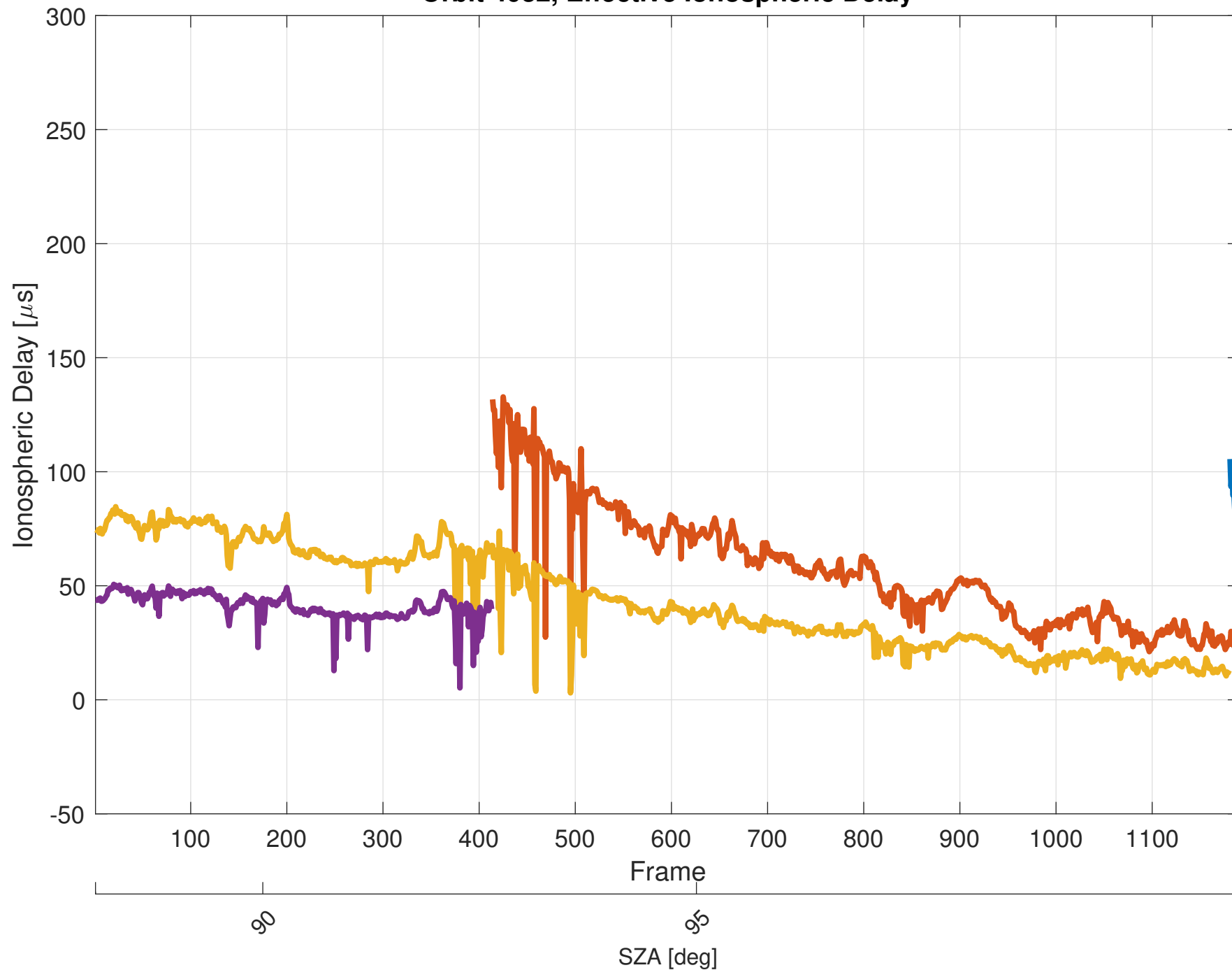
Orbit 4032, Effective Ionospheric Delay
