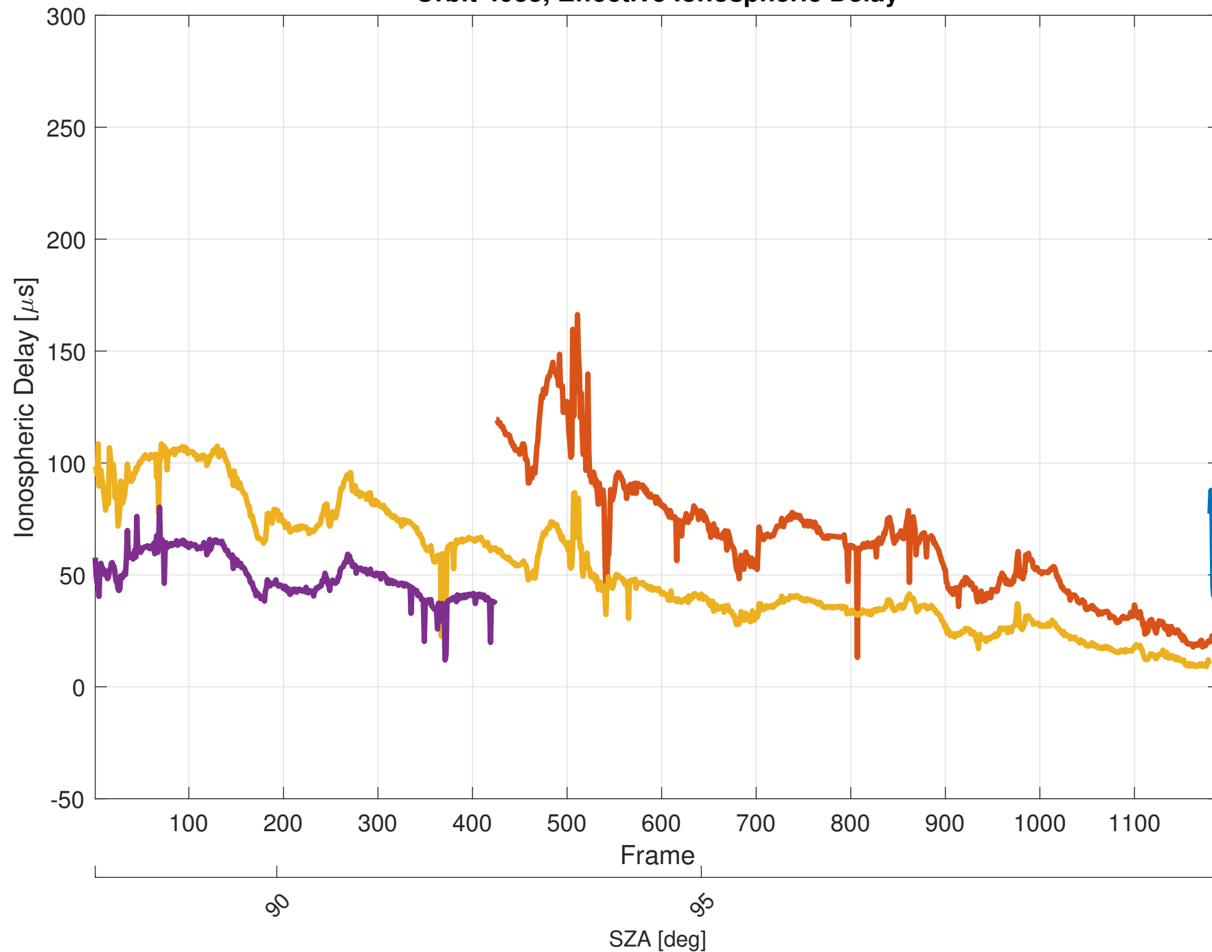
Orbit 4033, Effective Ionospheric Delay
