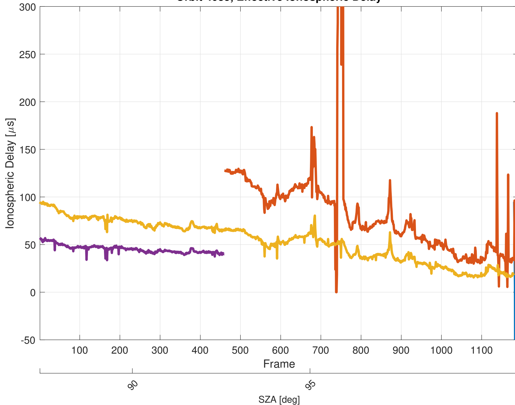
Orbit 4035, Effective Ionospheric Delay
