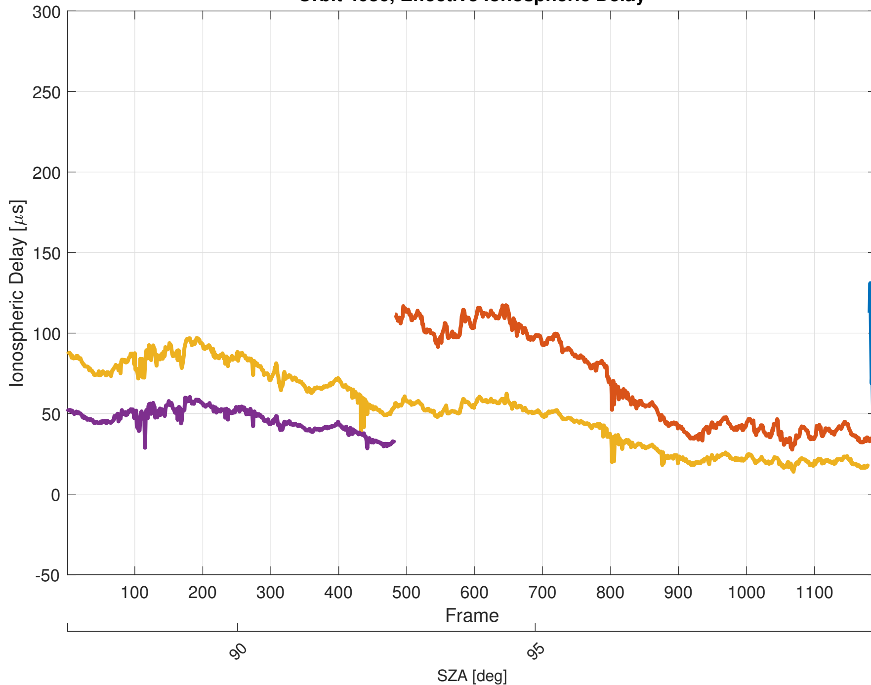
Orbit 4036, Effective Ionospheric Delay
