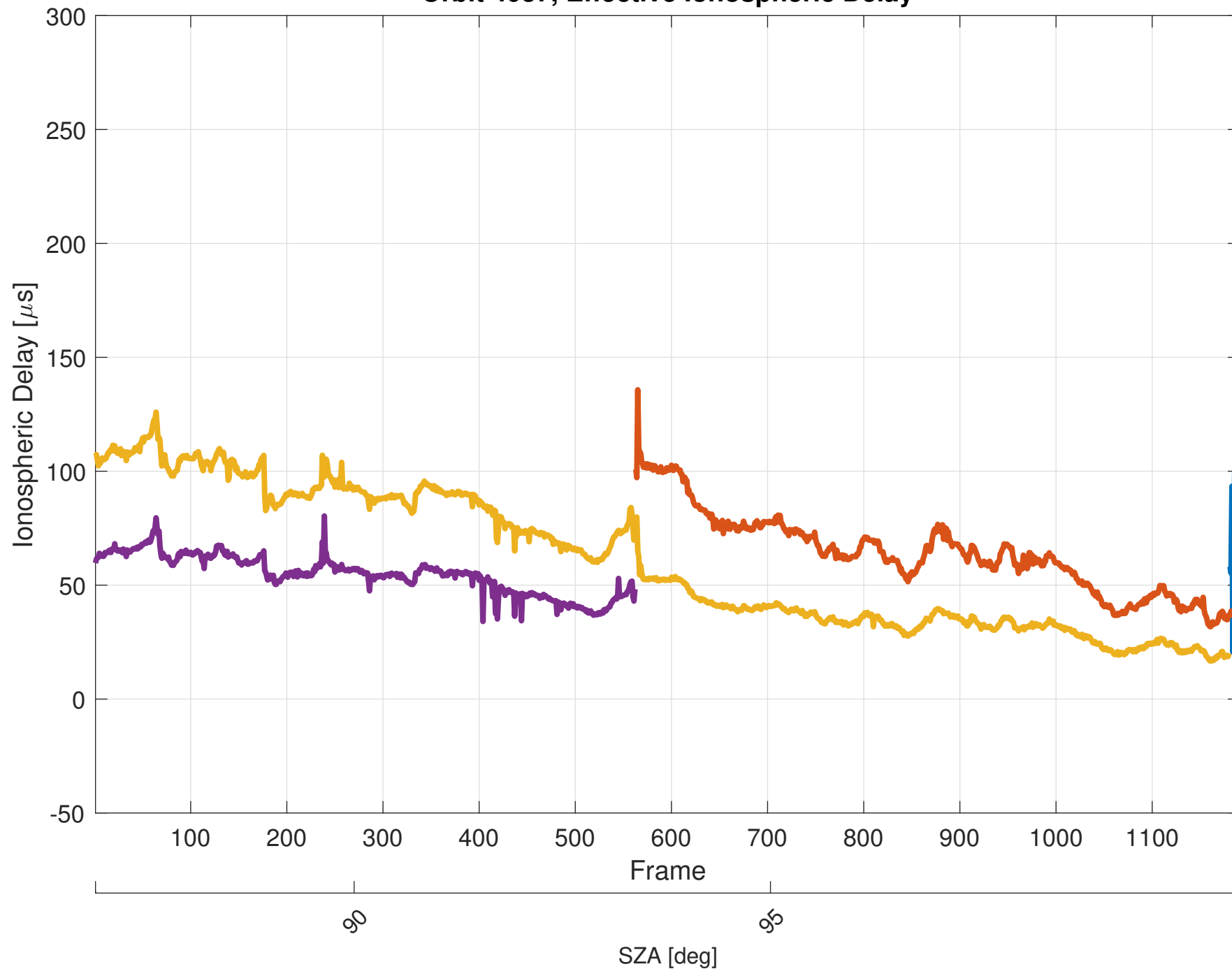
Orbit 4037, Effective Ionospheric Delay
