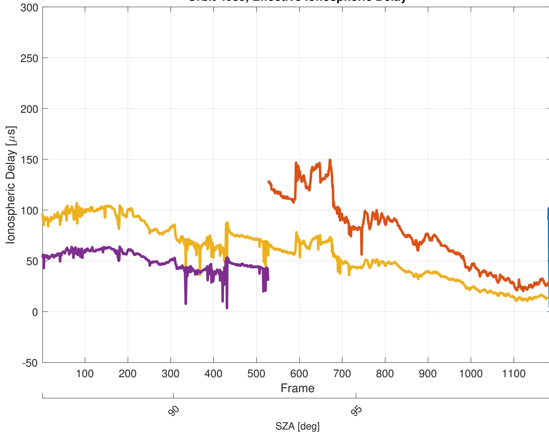
Orbit 4039, Effective Ionospheric Delay
