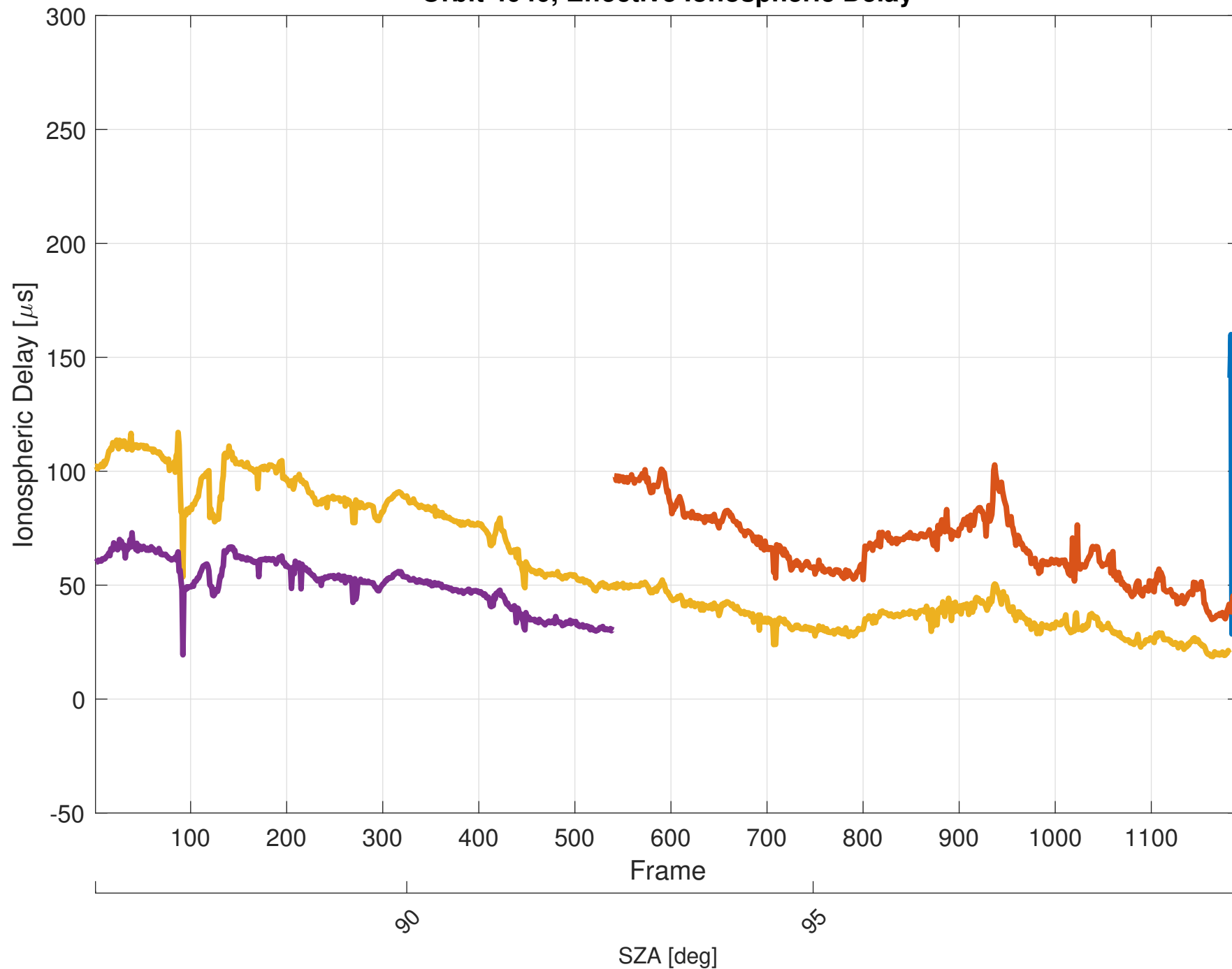
Orbit 4040, Effective Ionospheric Delay
