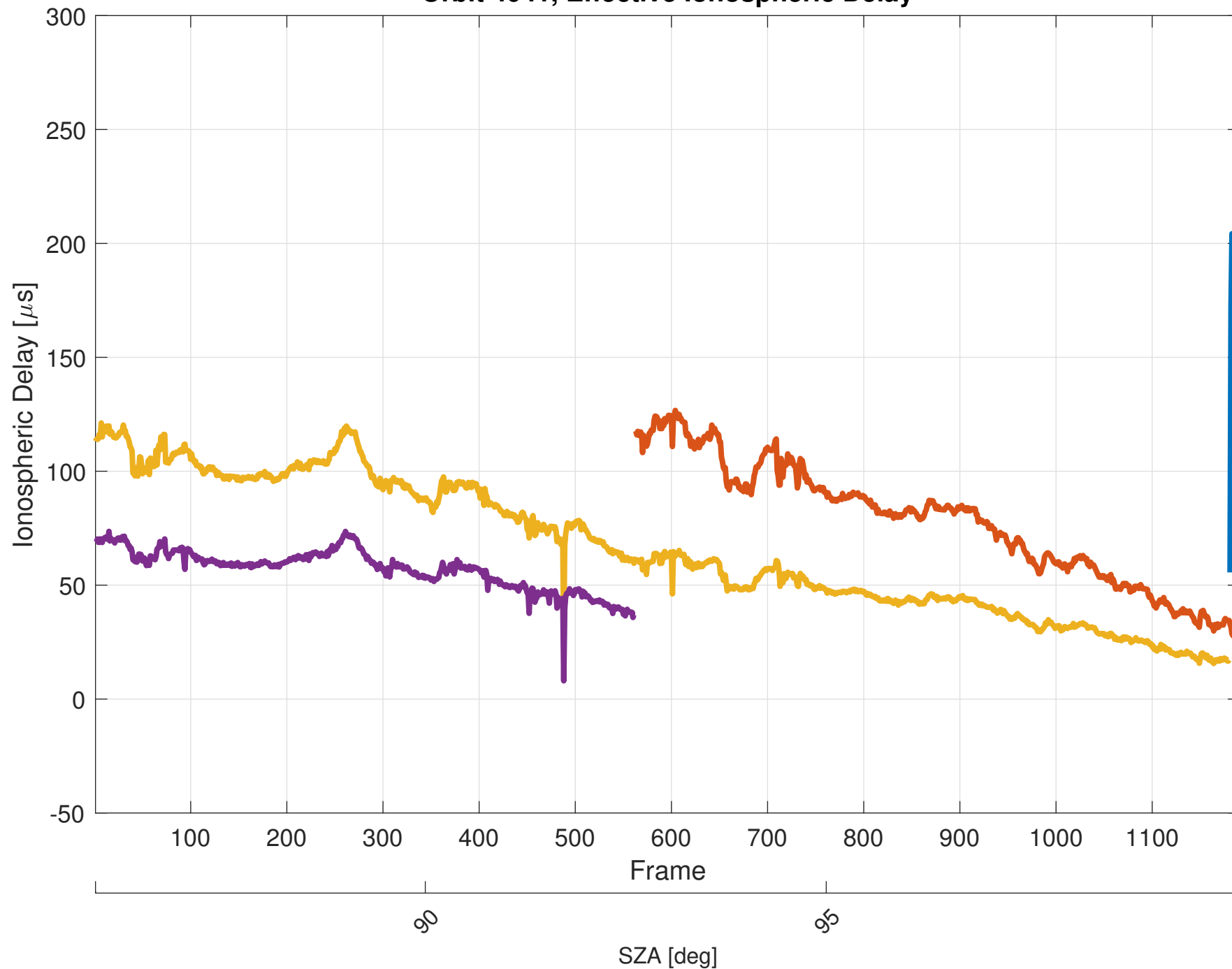
Orbit 4041, Effective Ionospheric Delay
