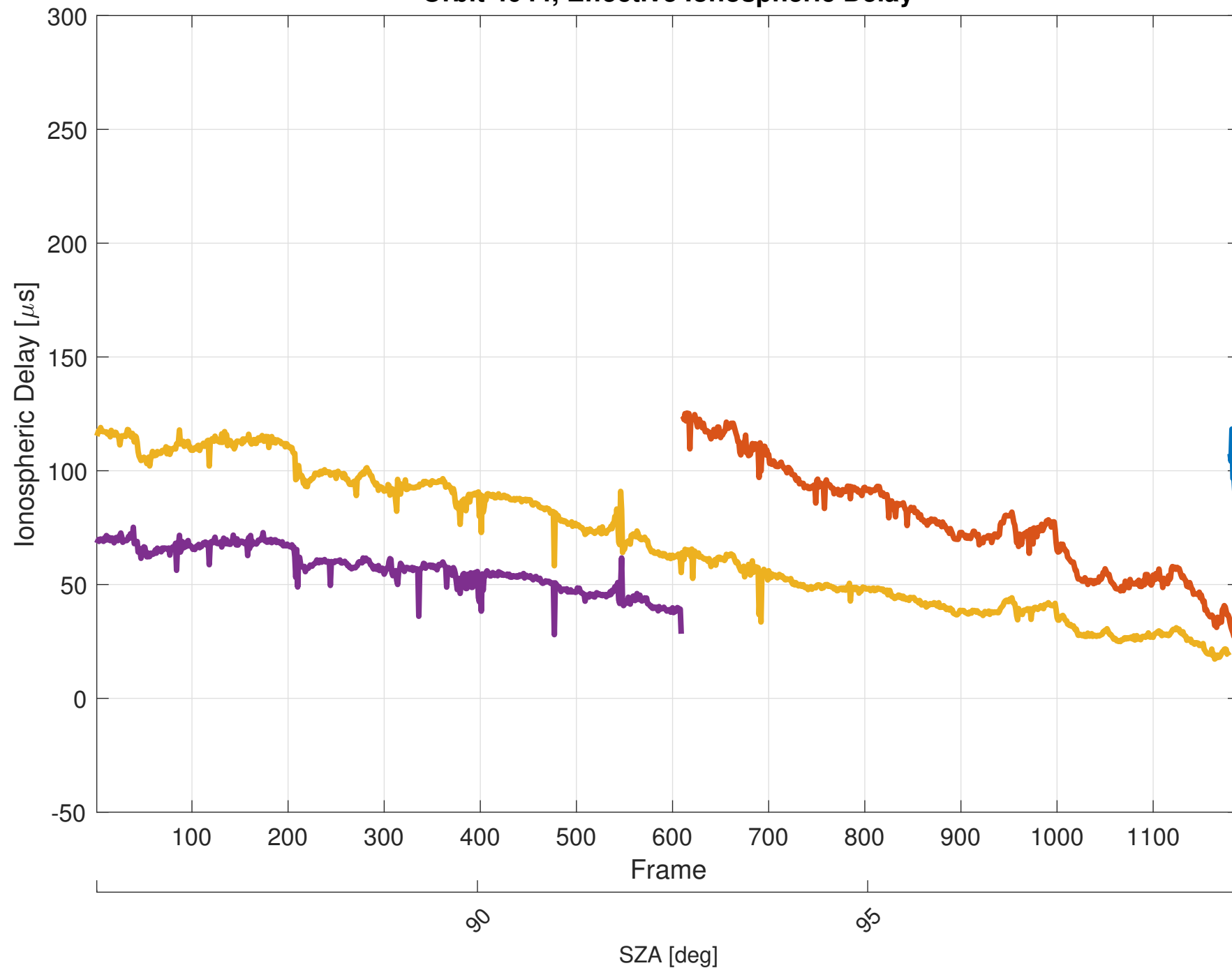
Orbit 4044, Effective Ionospheric Delay
