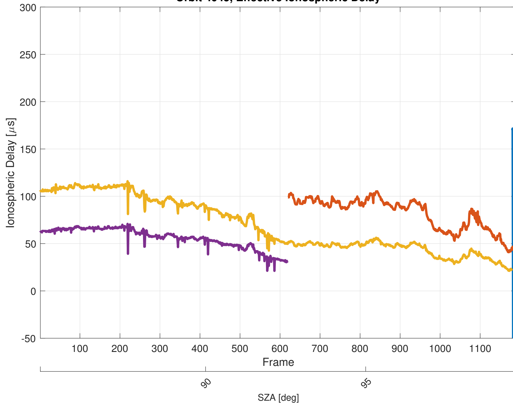
Orbit 4045, Effective Ionospheric Delay
