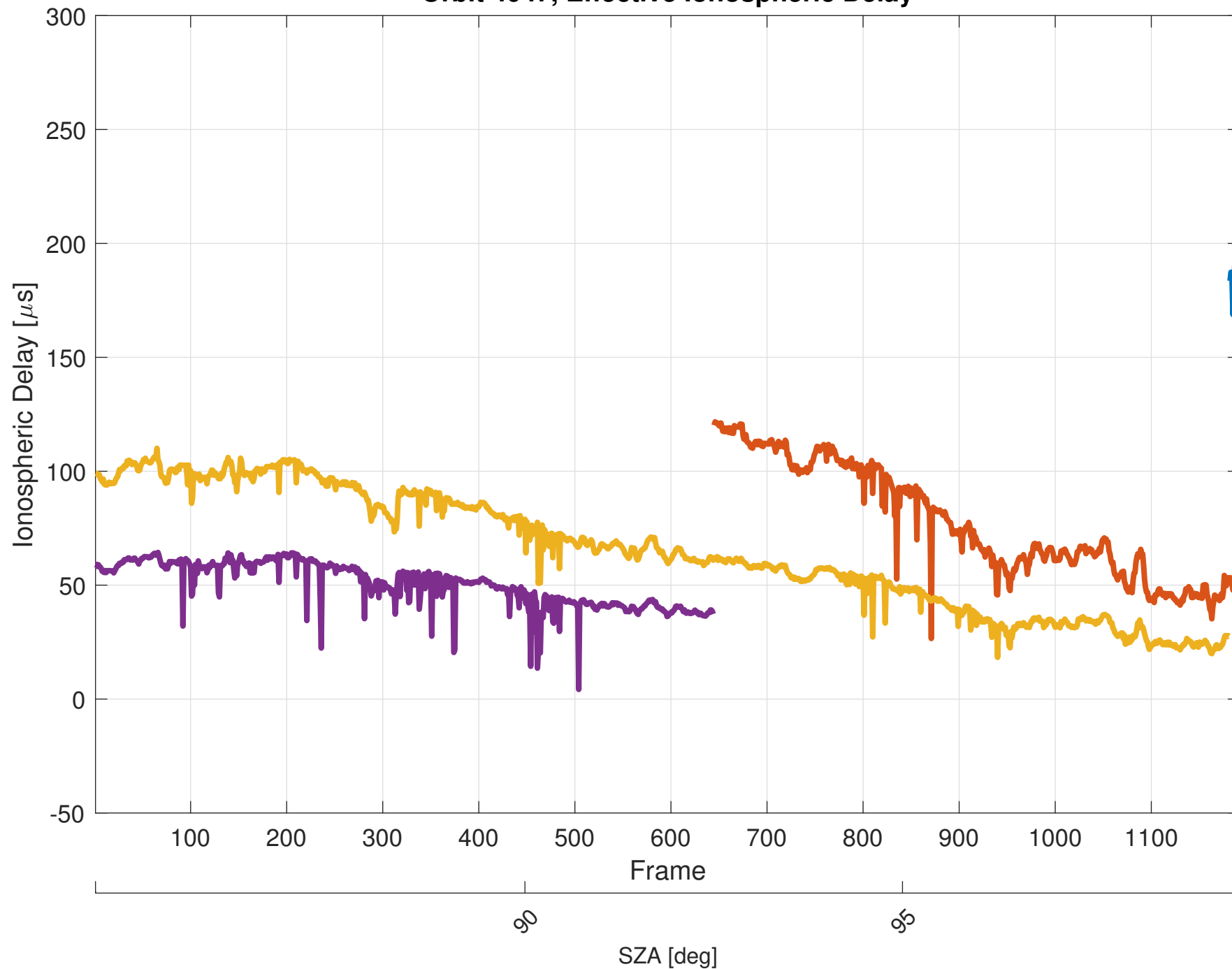
Orbit 4047, Effective Ionospheric Delay
