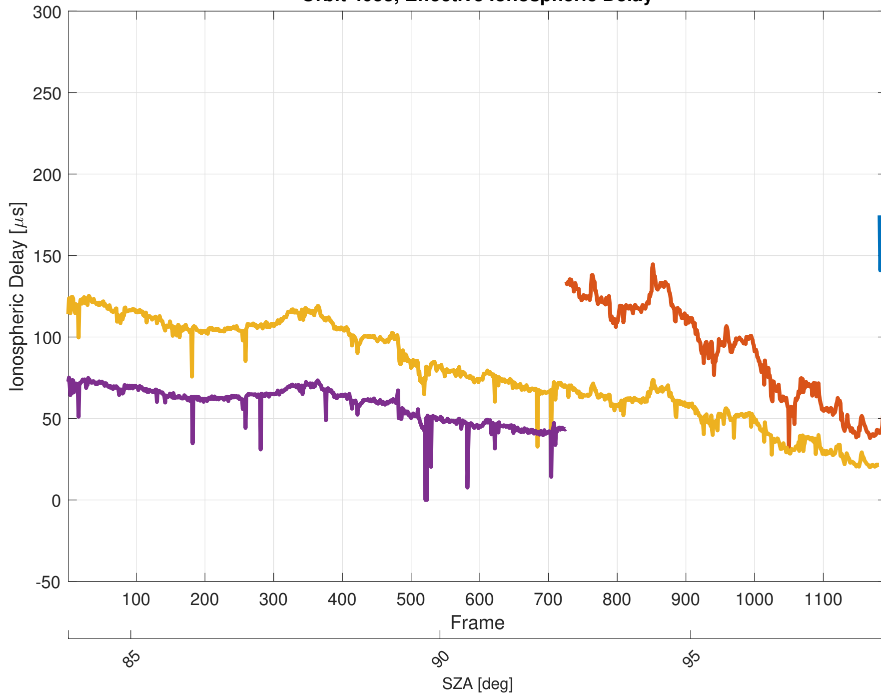
Orbit 4053, Effective Ionospheric Delay
