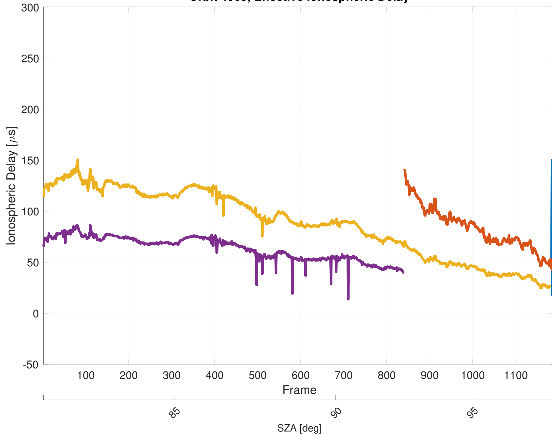
Orbit 4063, Effective Ionospheric Delay
