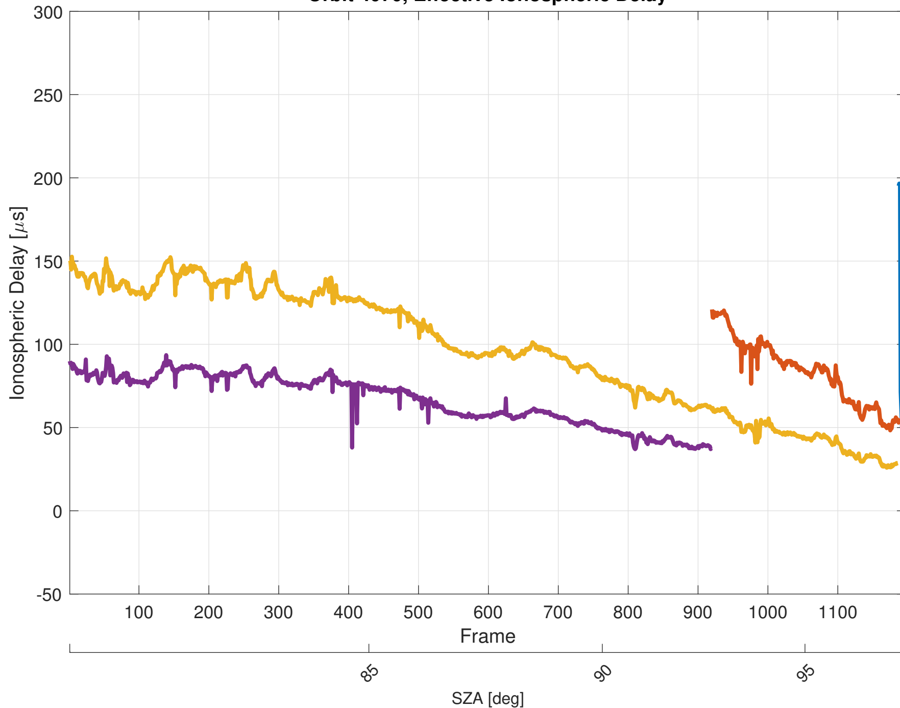
Orbit 4070, Effective Ionospheric Delay
