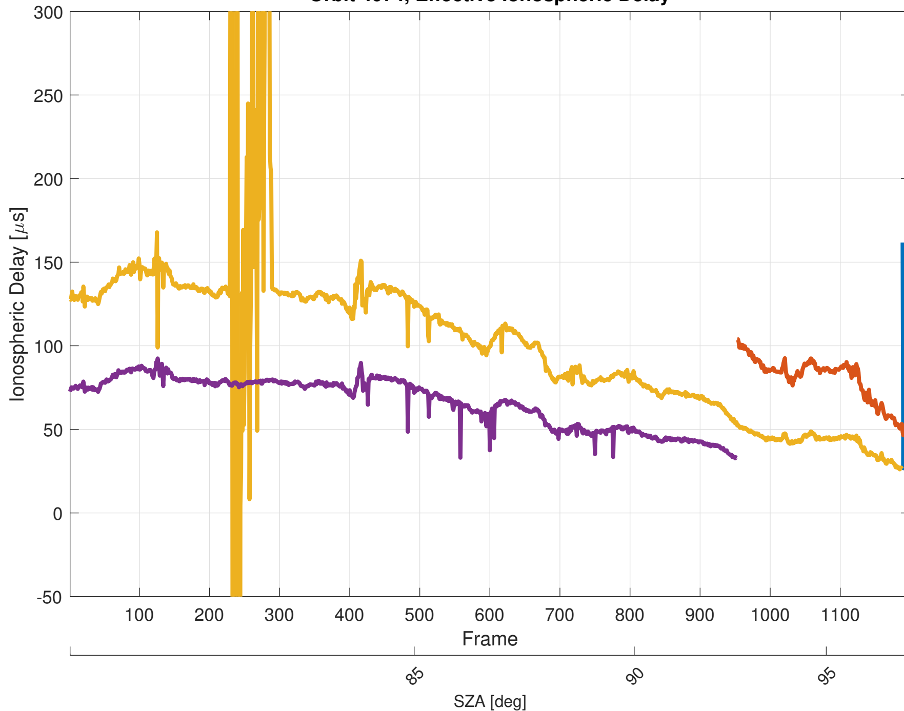
Orbit 4074, Effective Ionospheric Delay
