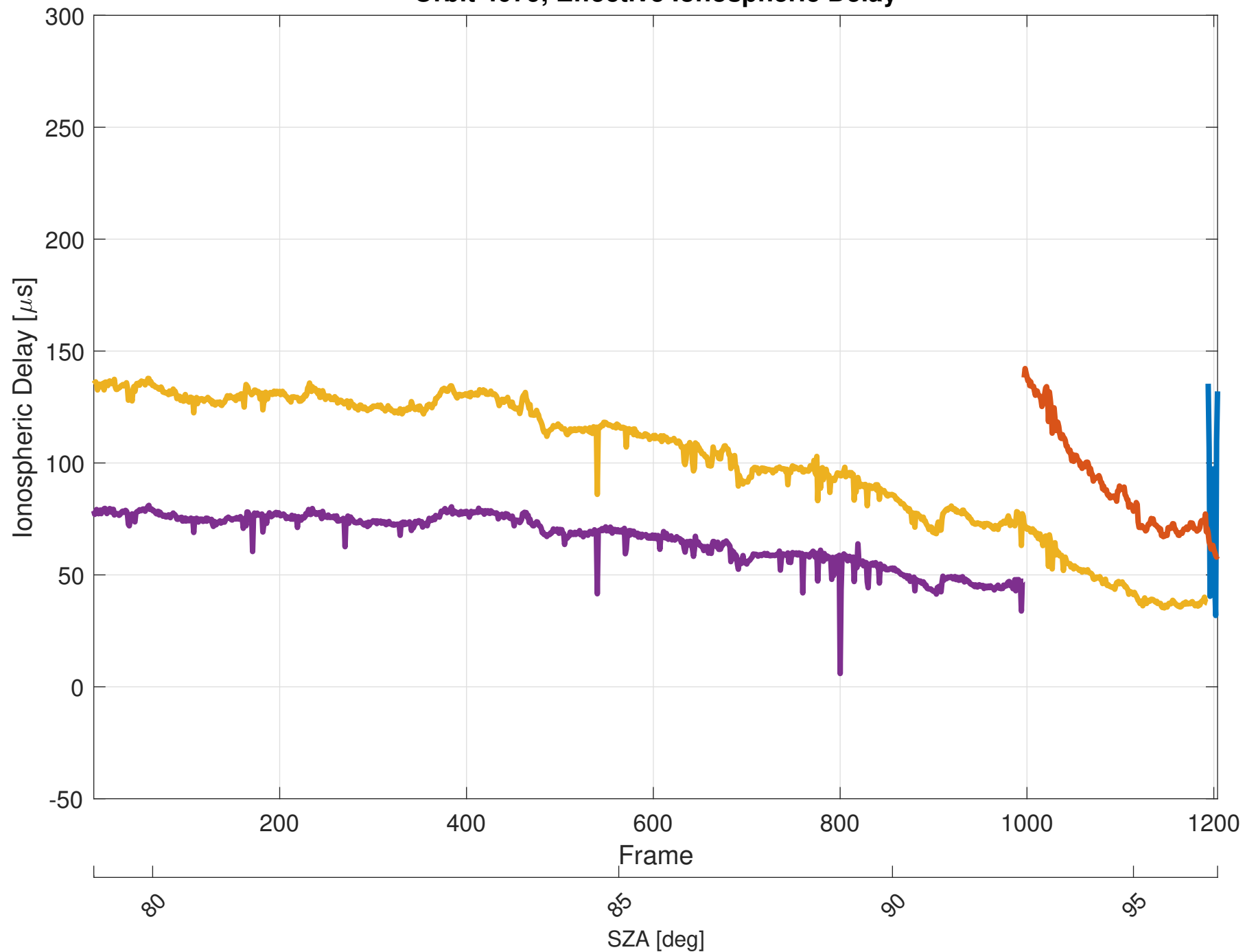
Orbit 4079, Effective Ionospheric Delay
