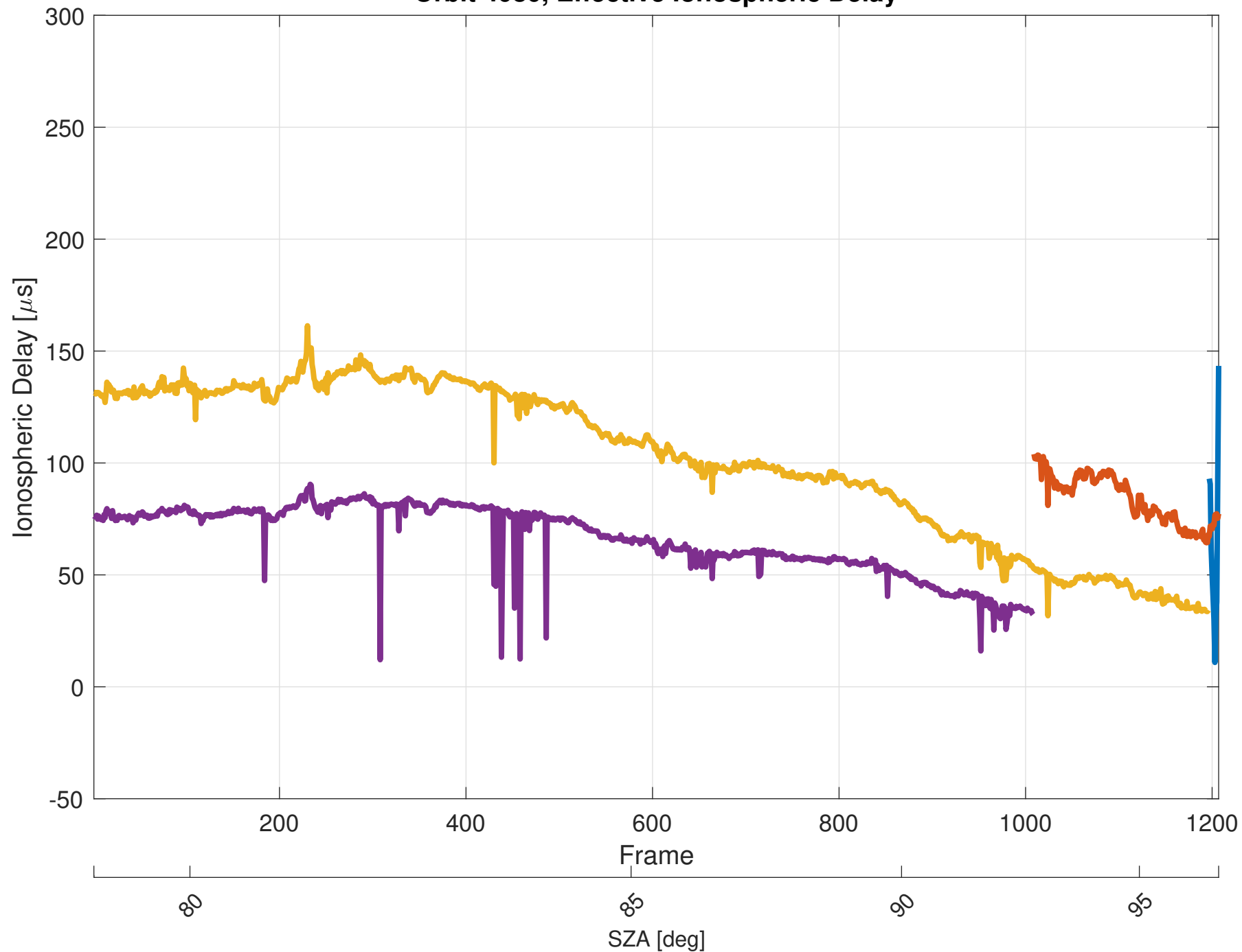
Orbit 4080, Effective Ionospheric Delay
