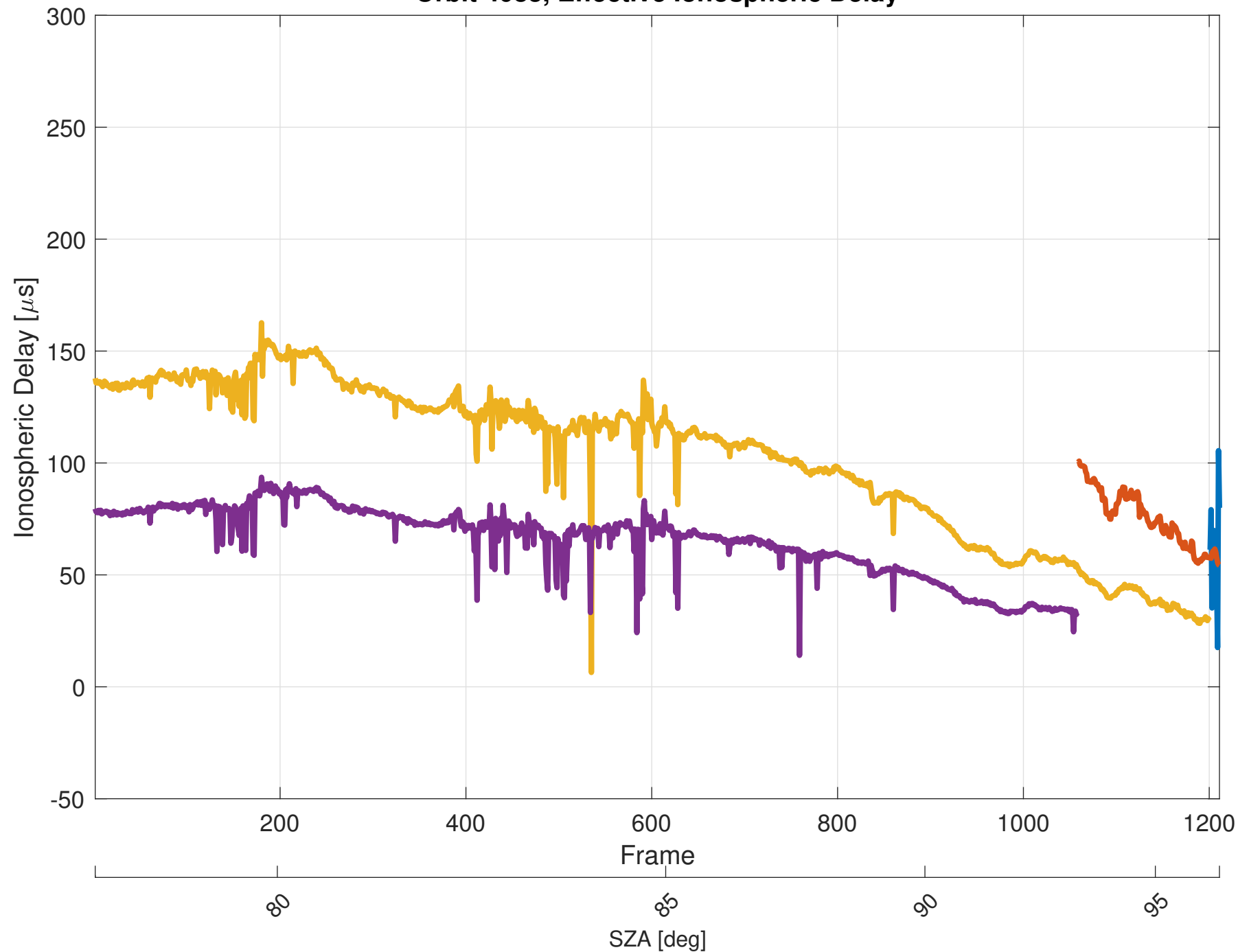
Orbit 4083, Effective Ionospheric Delay
