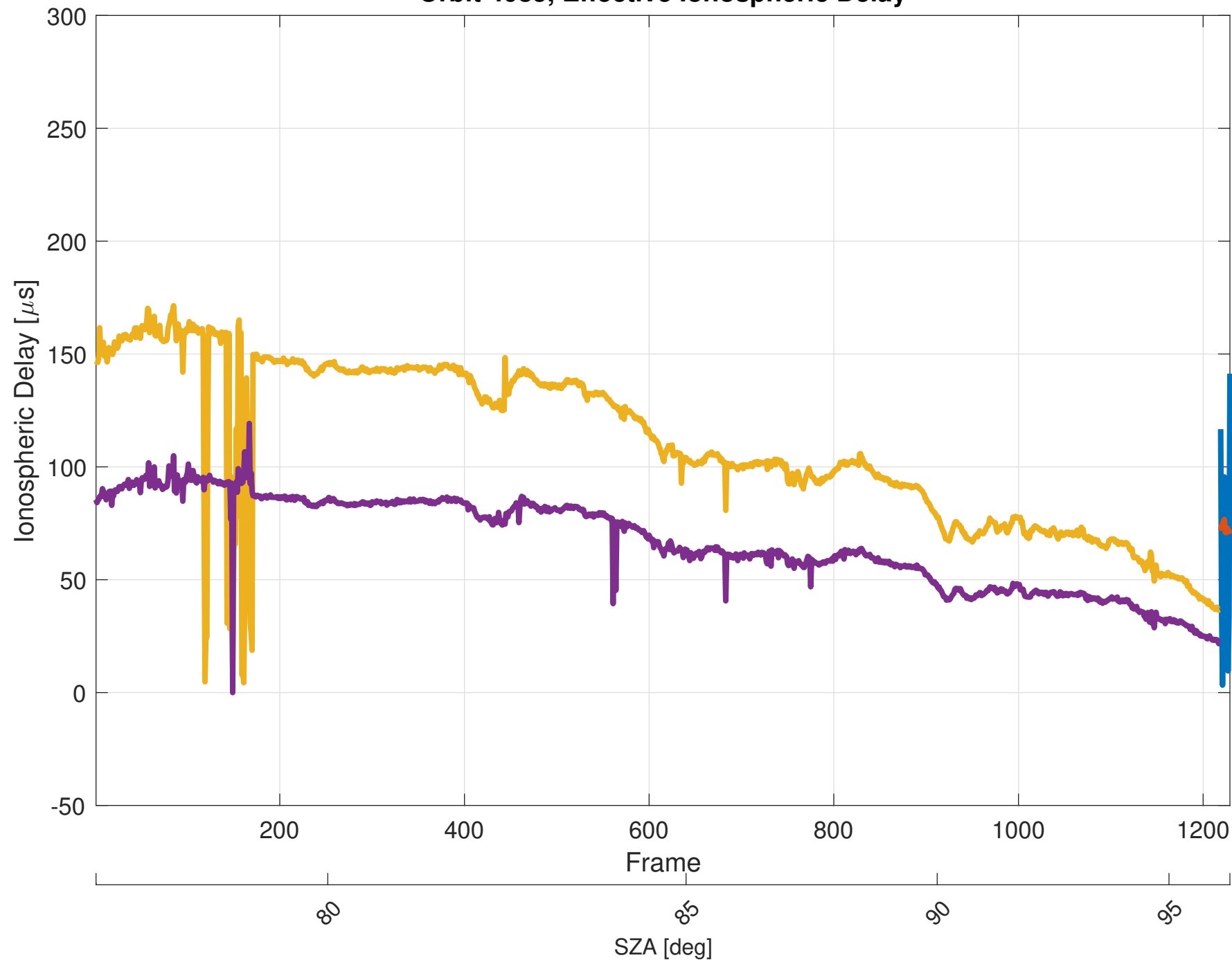
Orbit 4085, Effective Ionospheric Delay
