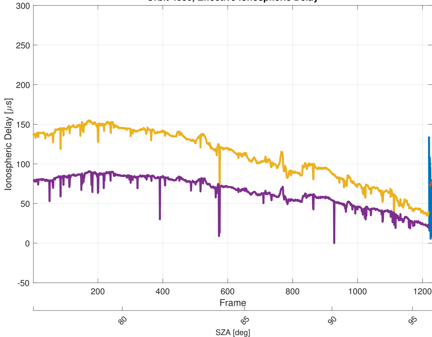
Orbit 4086, Effective Ionospheric Delay
