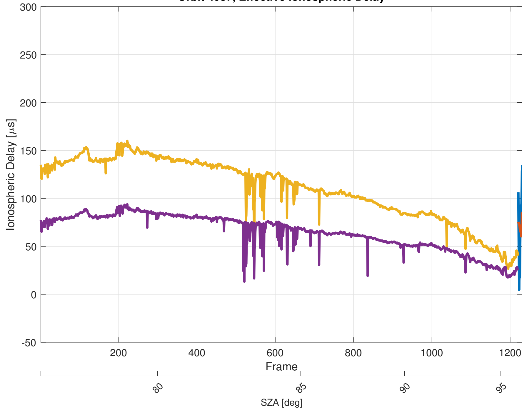
Orbit 4087, Effective Ionospheric Delay
