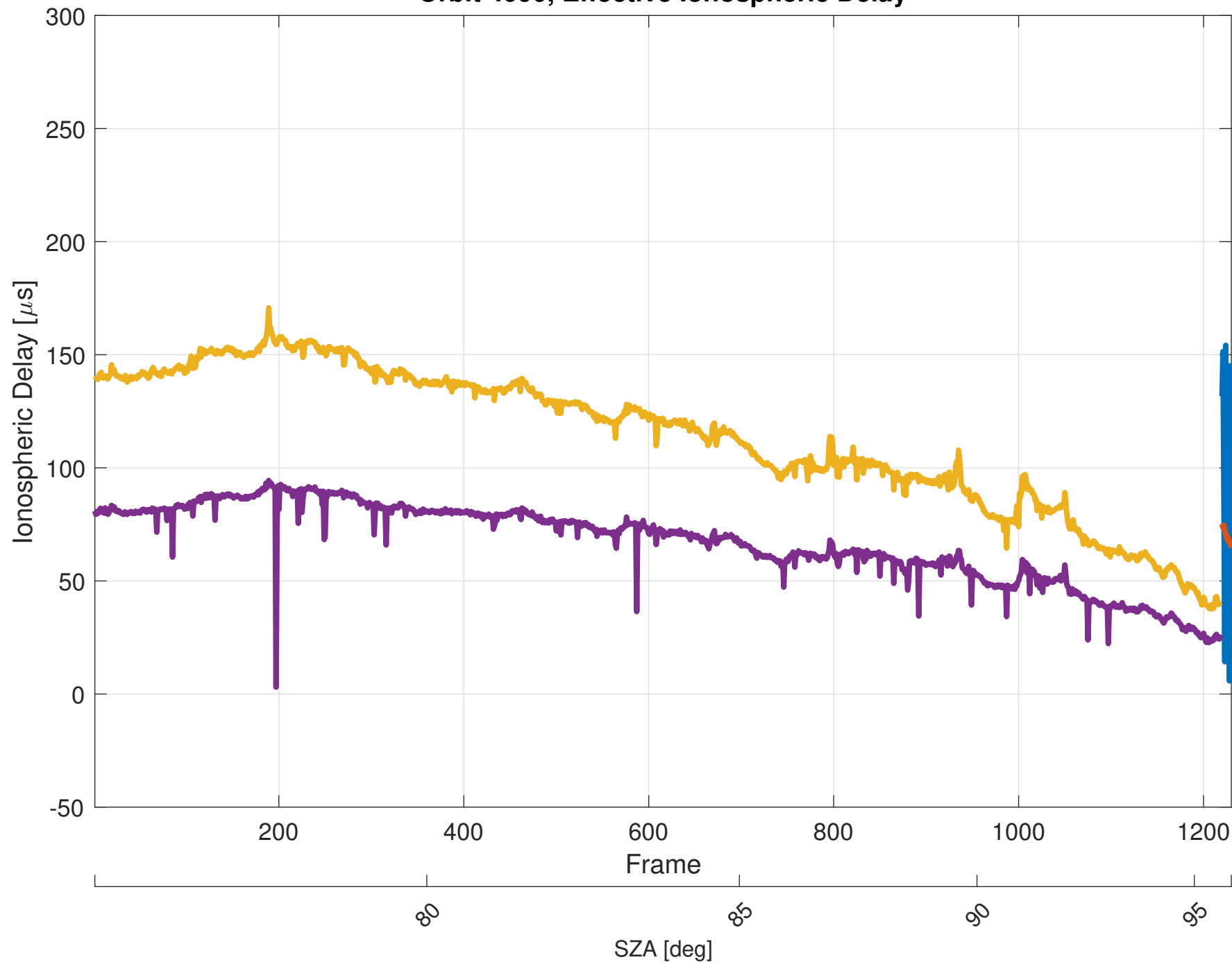
Orbit 4090, Effective Ionospheric Delay
