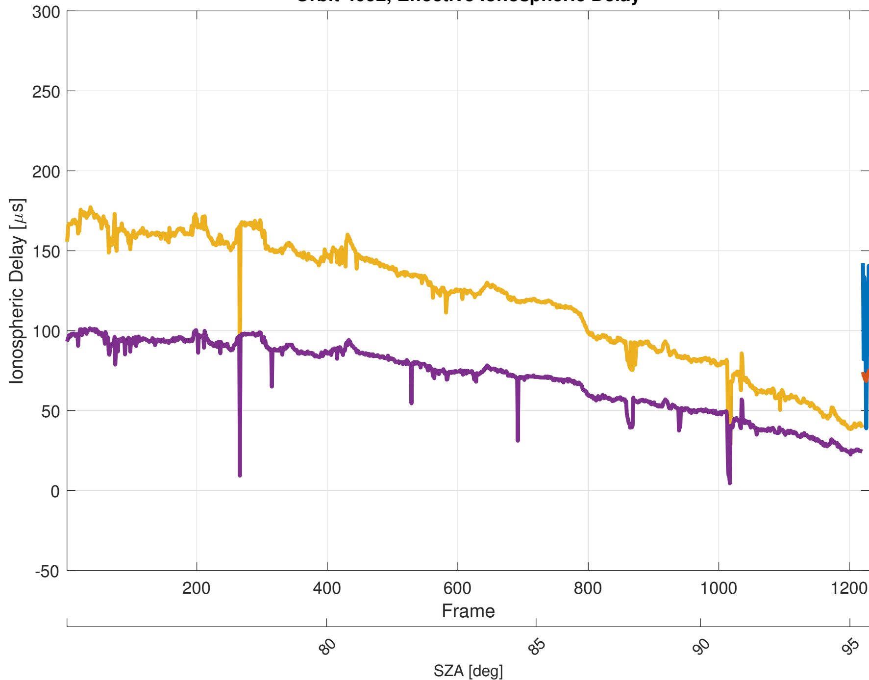
Orbit 4092, Effective Ionospheric Delay
