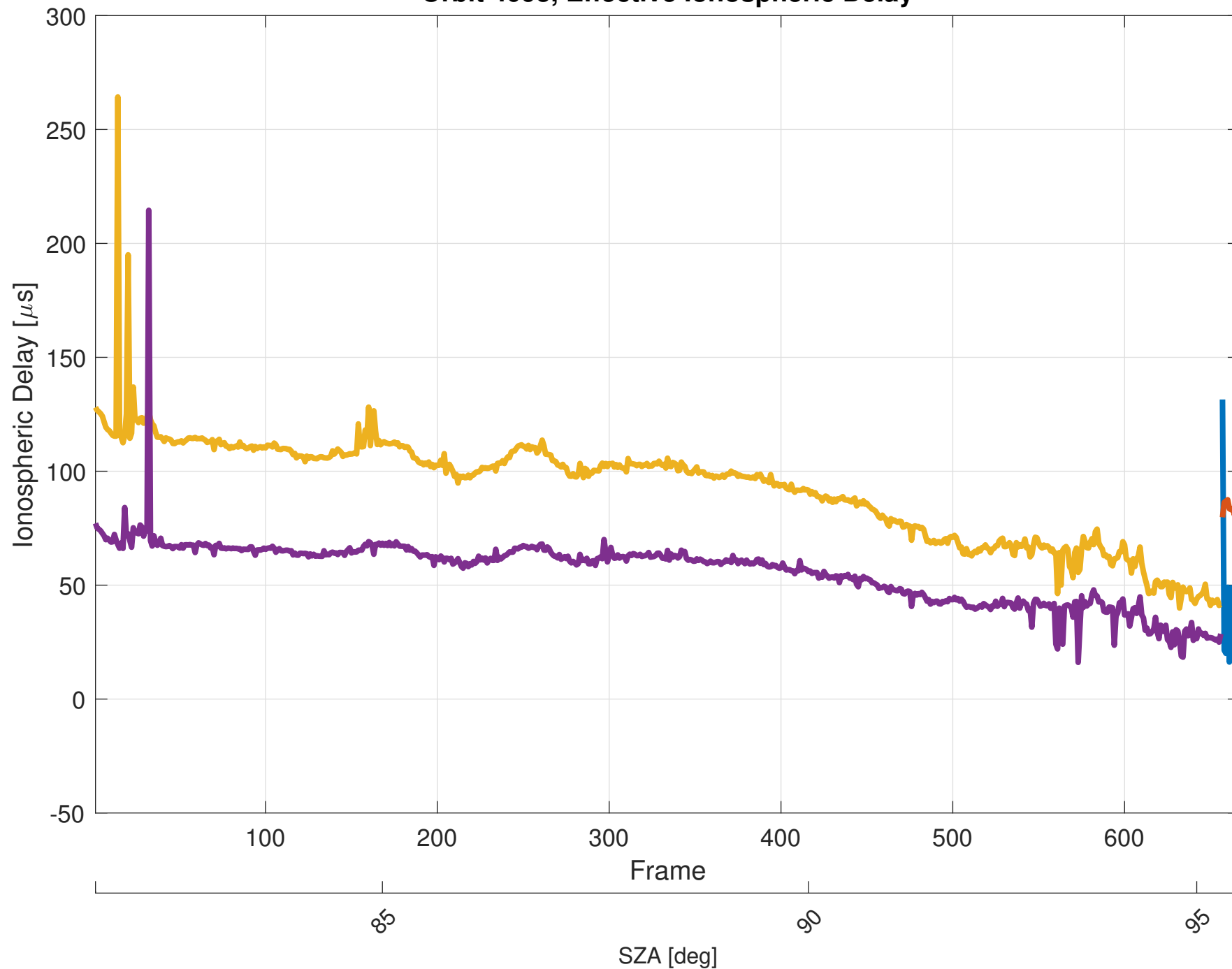
Orbit 4093, Effective Ionospheric Delay
