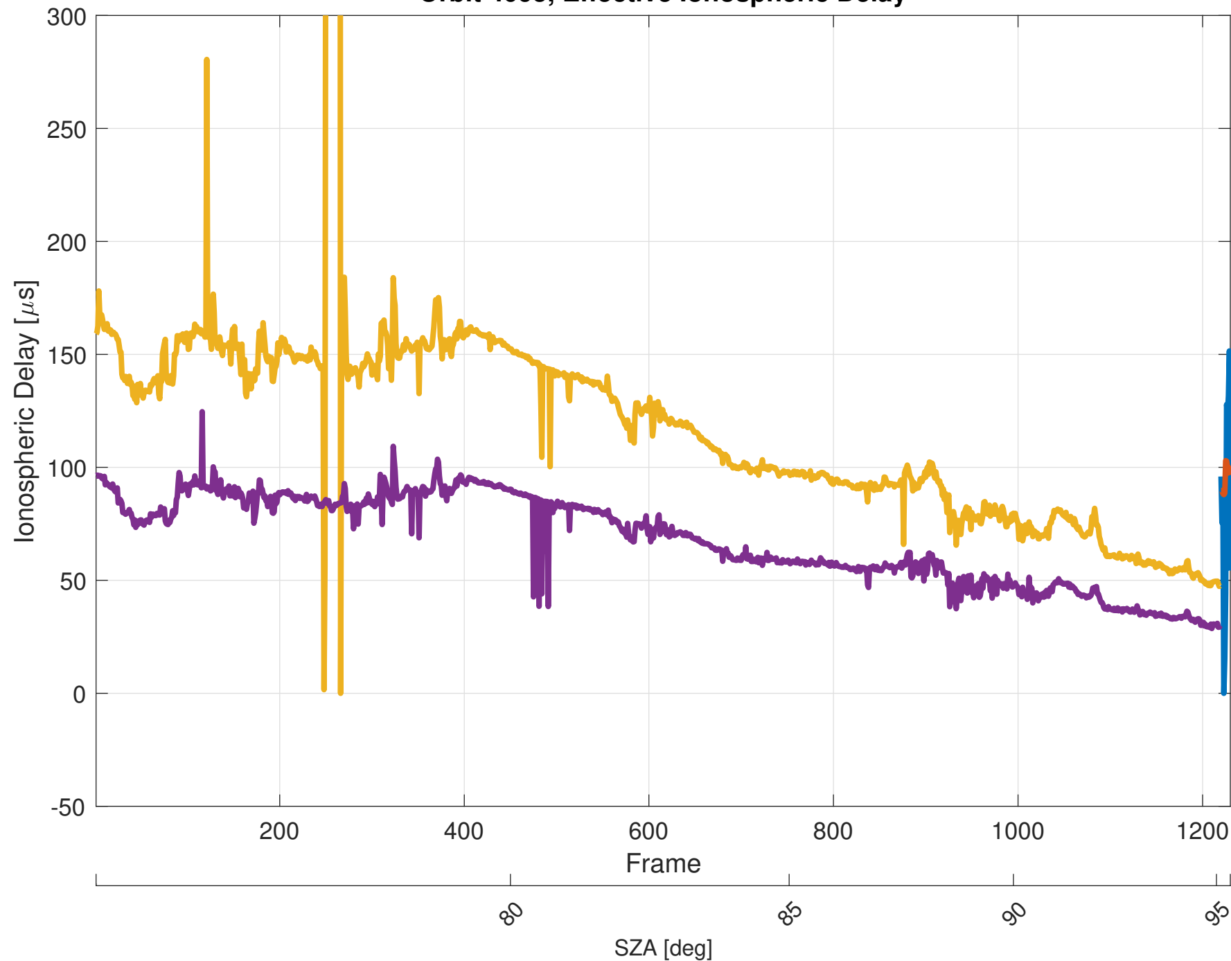
Orbit 4095, Effective Ionospheric Delay
