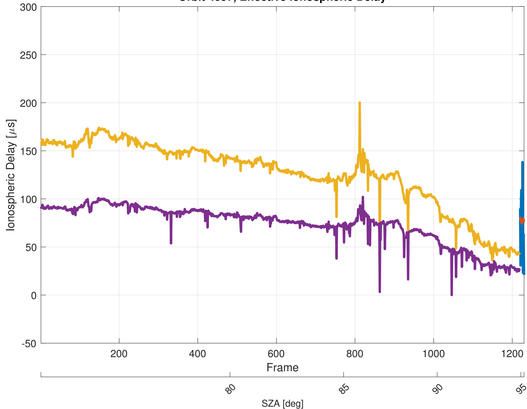
Orbit 4097, Effective Ionospheric Delay
