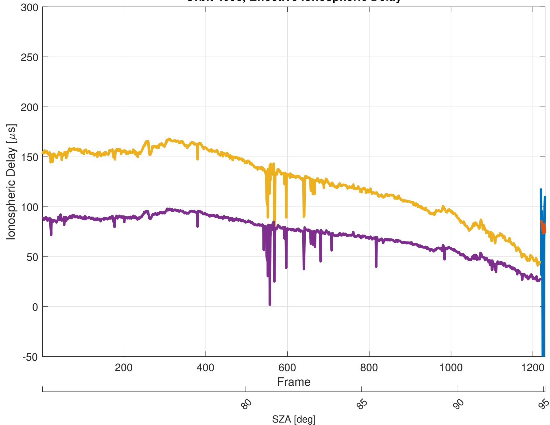
Orbit 4098, Effective Ionospheric Delay
