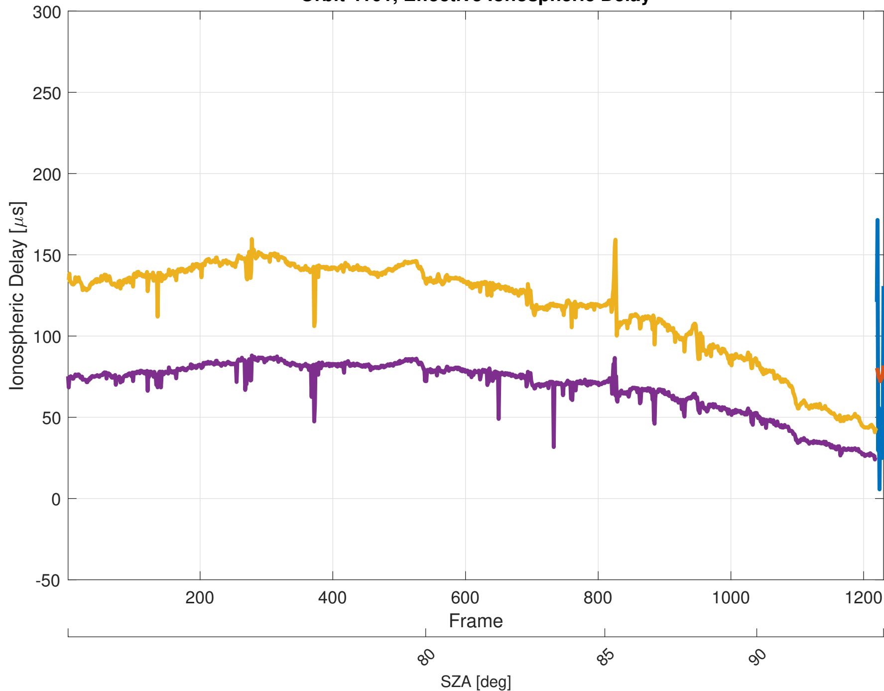
Orbit 4101, Effective Ionospheric Delay
