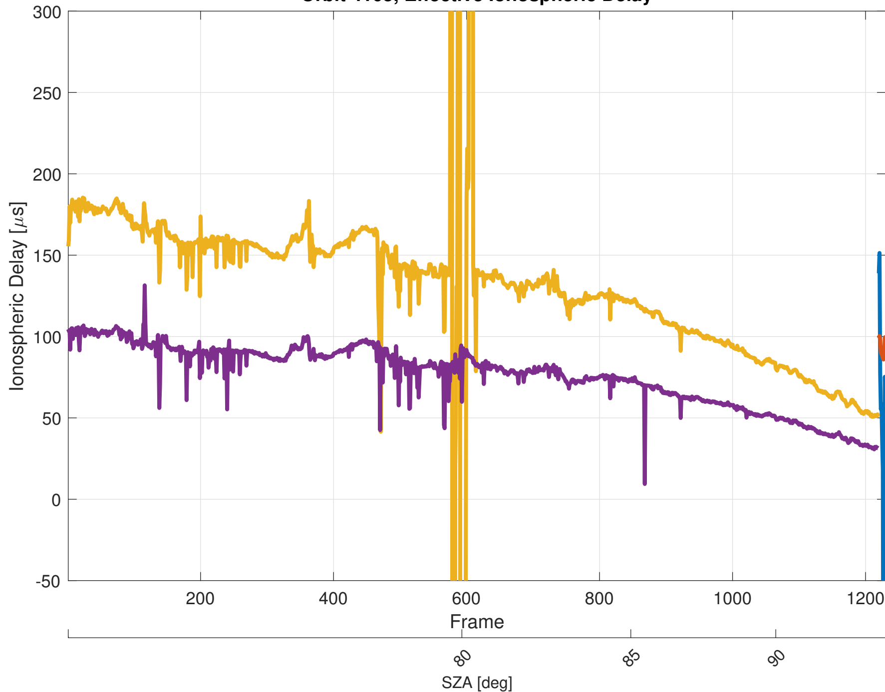
Orbit 4105, Effective Ionospheric Delay
