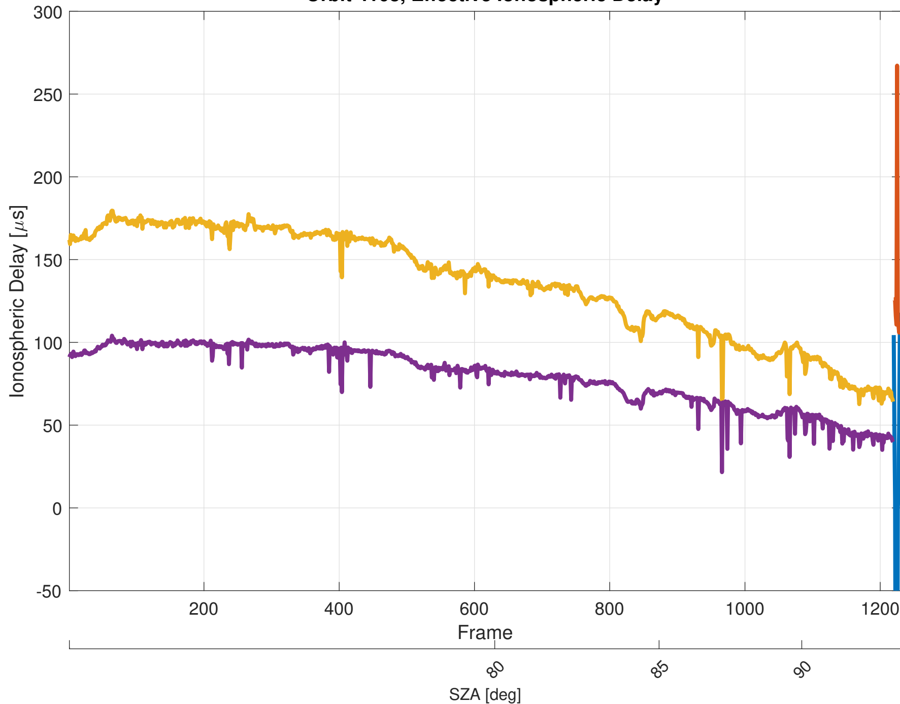
Orbit 4108, Effective Ionospheric Delay
