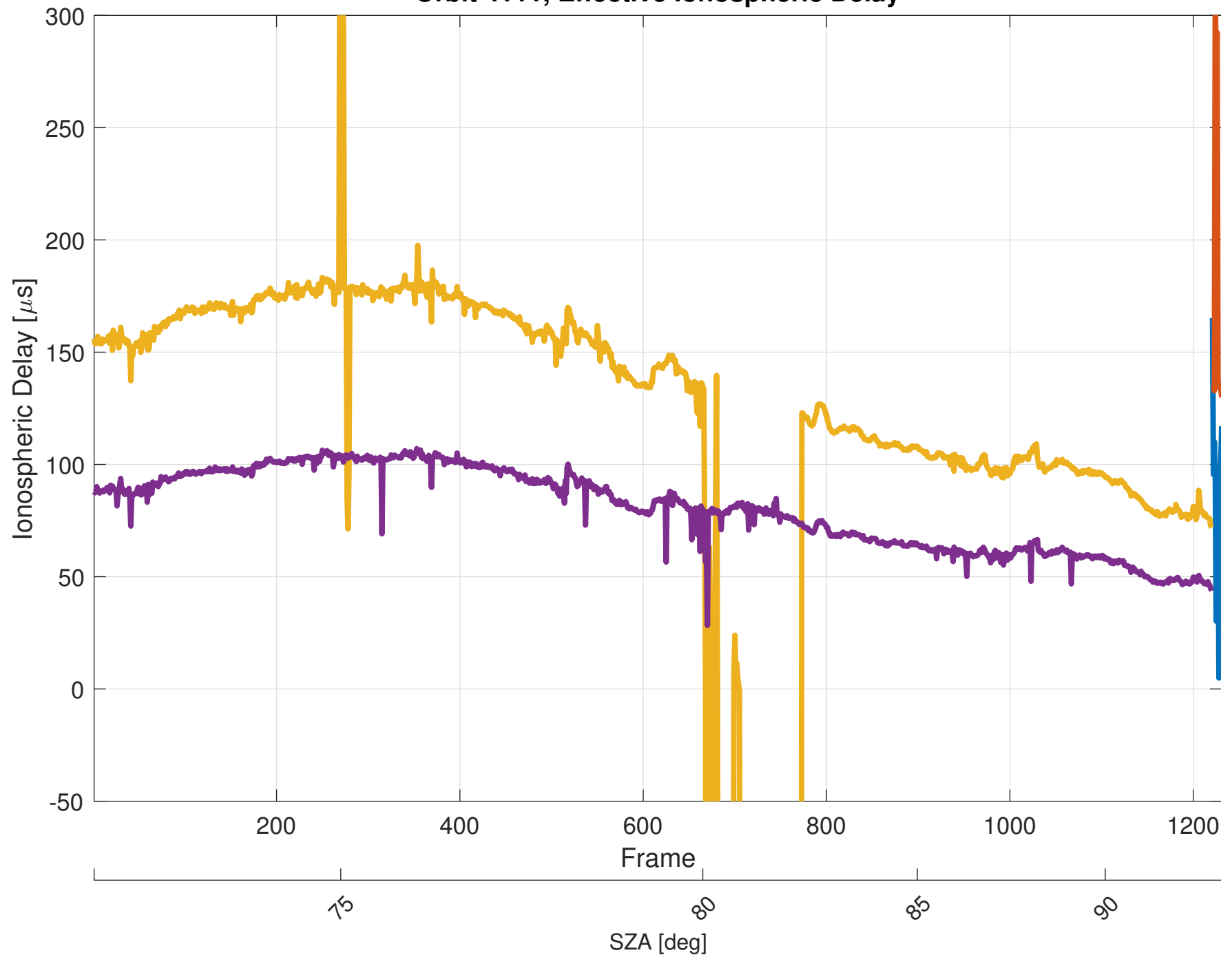
Orbit 4111, Effective Ionospheric Delay
