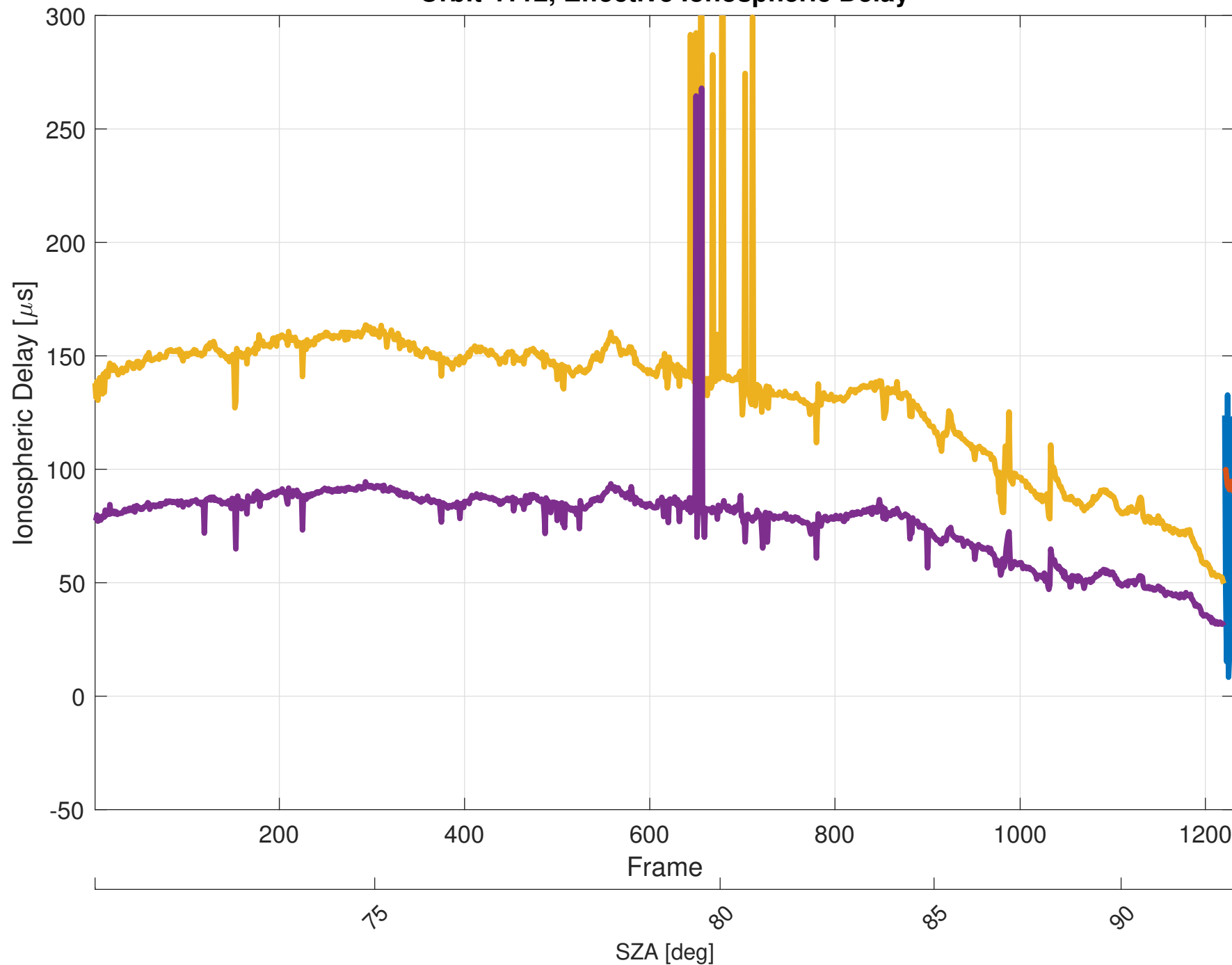
Orbit 4112, Effective Ionospheric Delay
