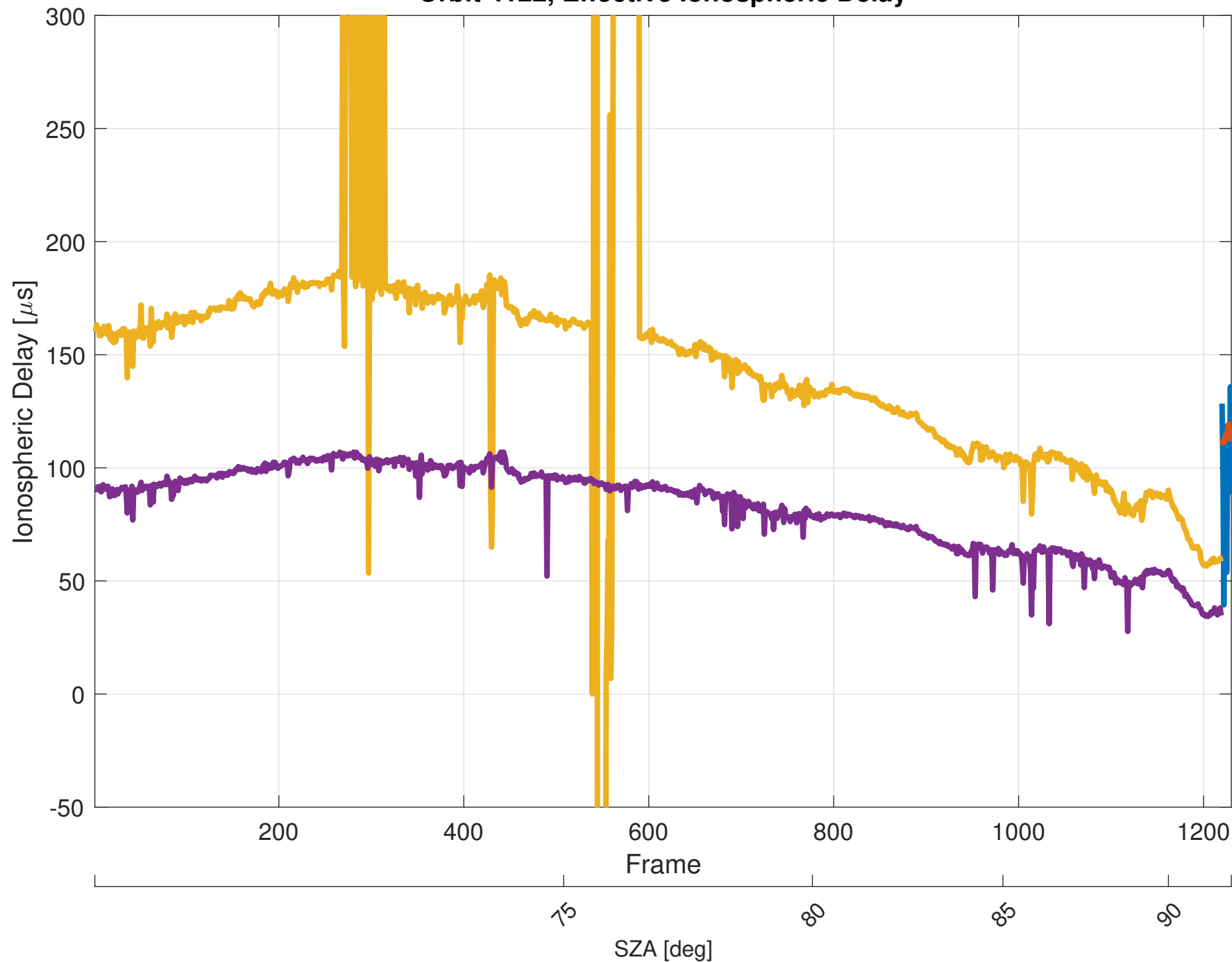
Orbit 4122, Effective Ionospheric Delay
