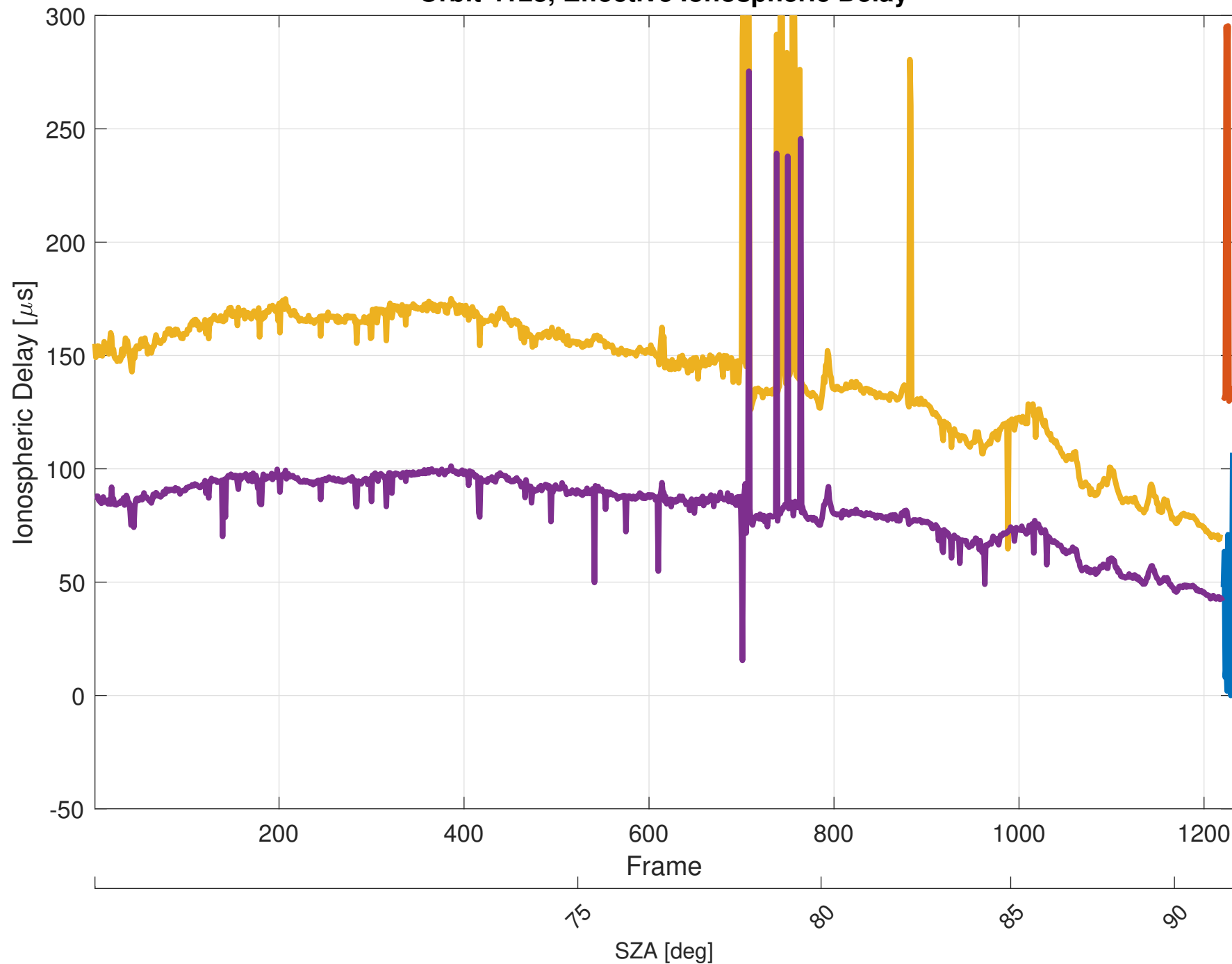
Orbit 4123, Effective Ionospheric Delay
