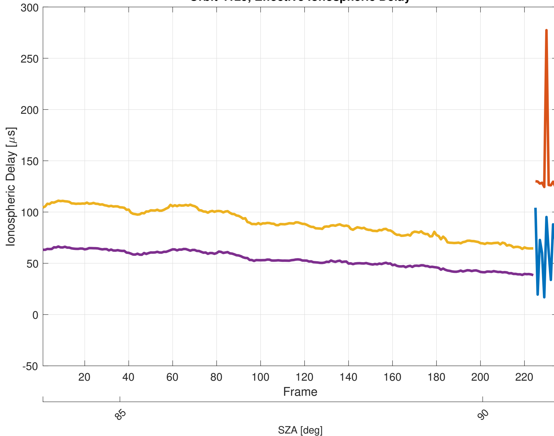
Orbit 4129, Effective Ionospheric Delay
