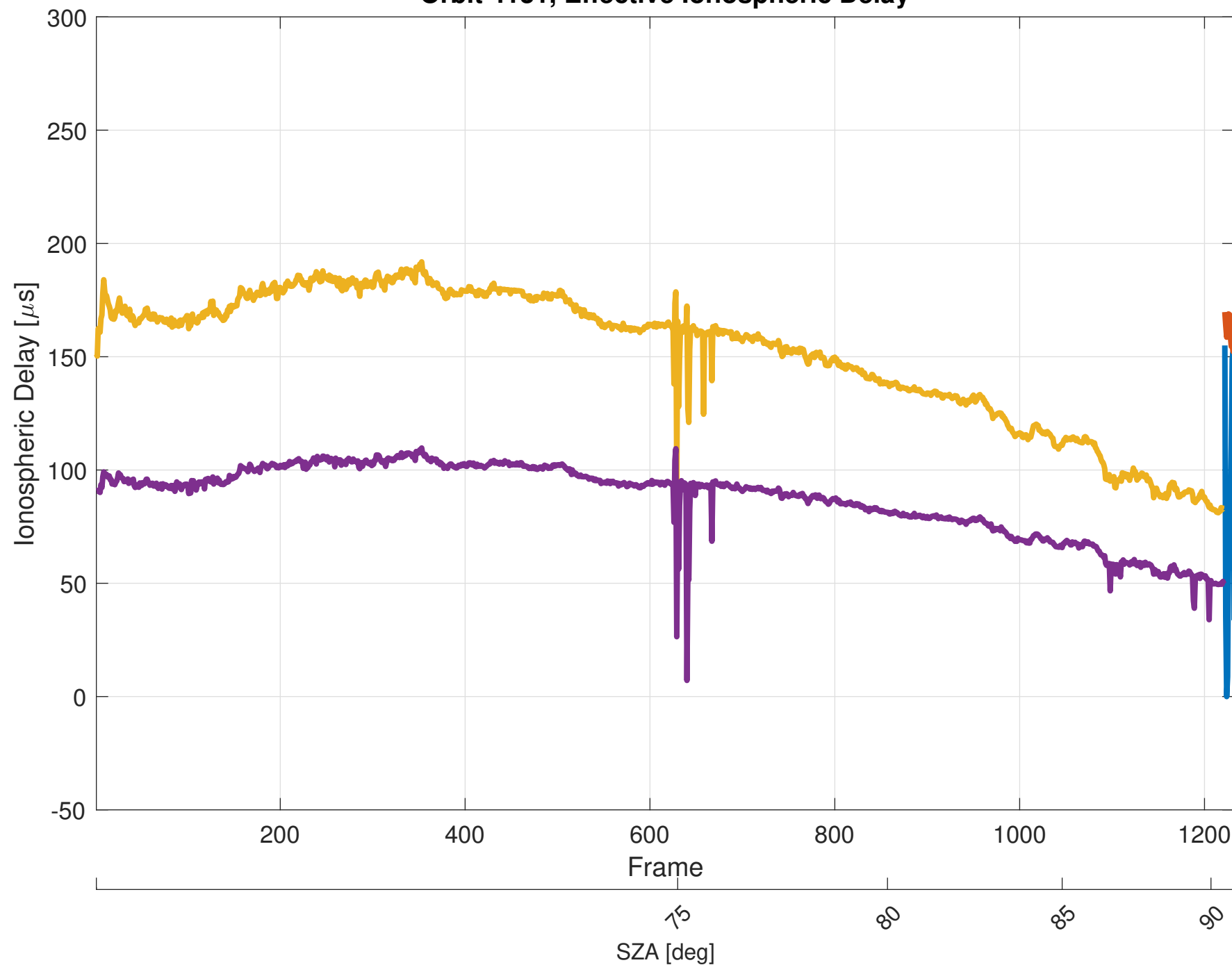
Orbit 4131, Effective Ionospheric Delay
