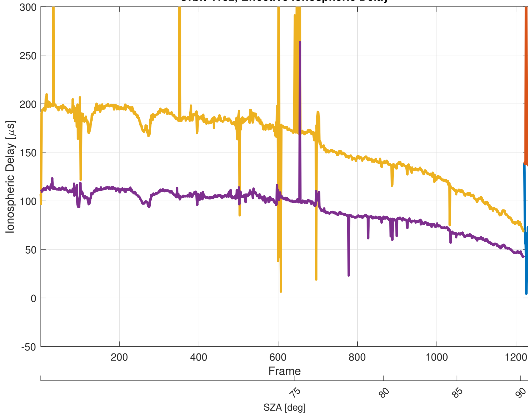
Orbit 4132, Effective Ionospheric Delay
