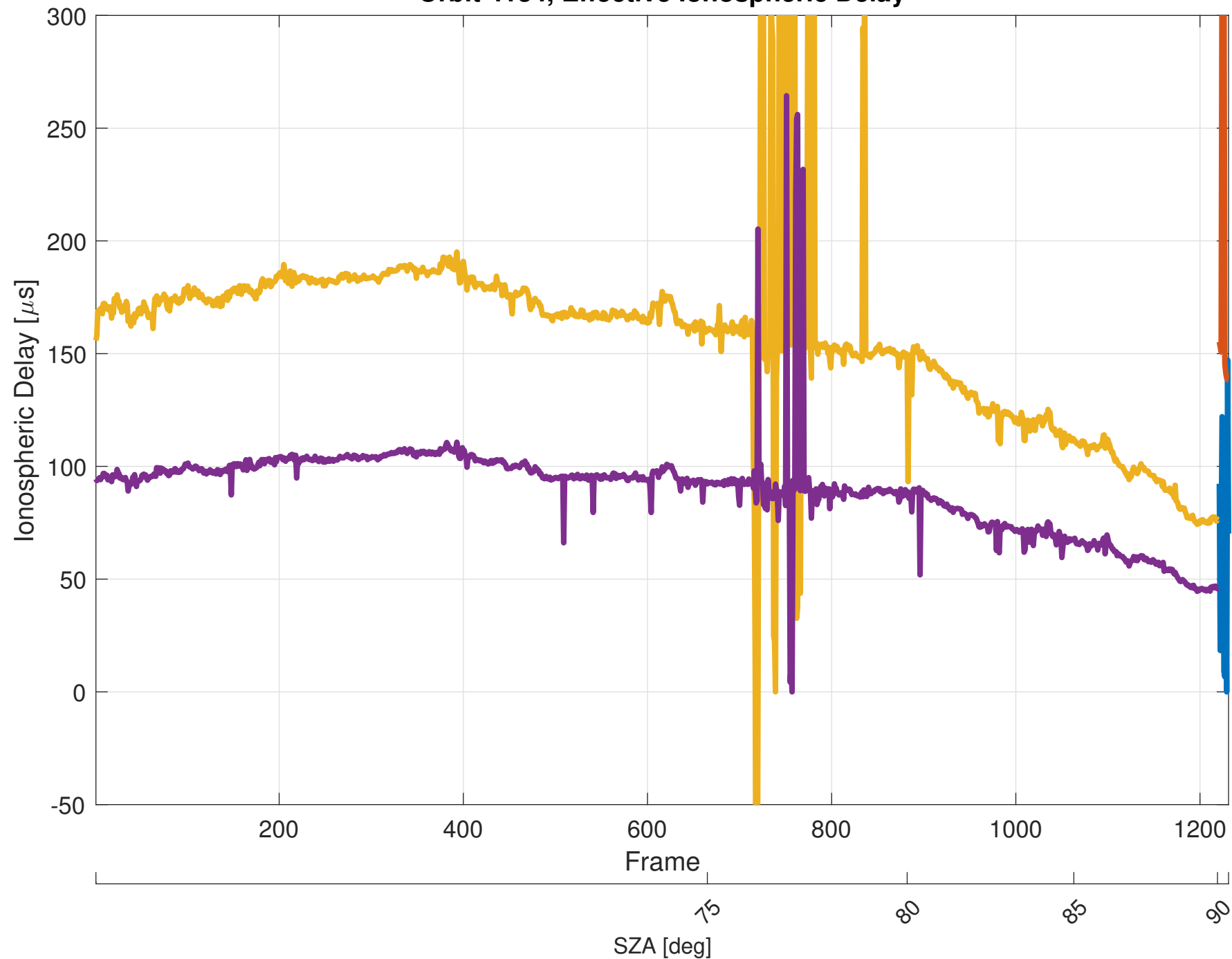
Orbit 4134, Effective Ionospheric Delay
