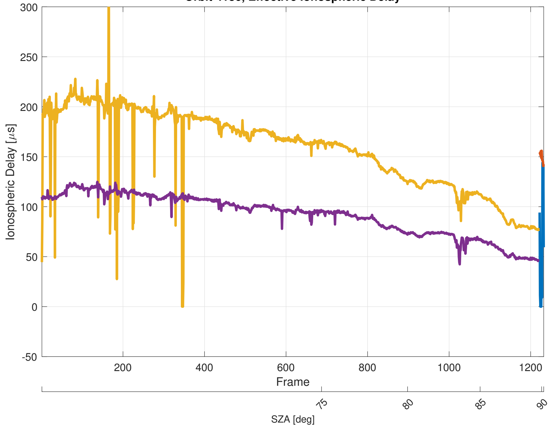
Orbit 4136, Effective Ionospheric Delay
