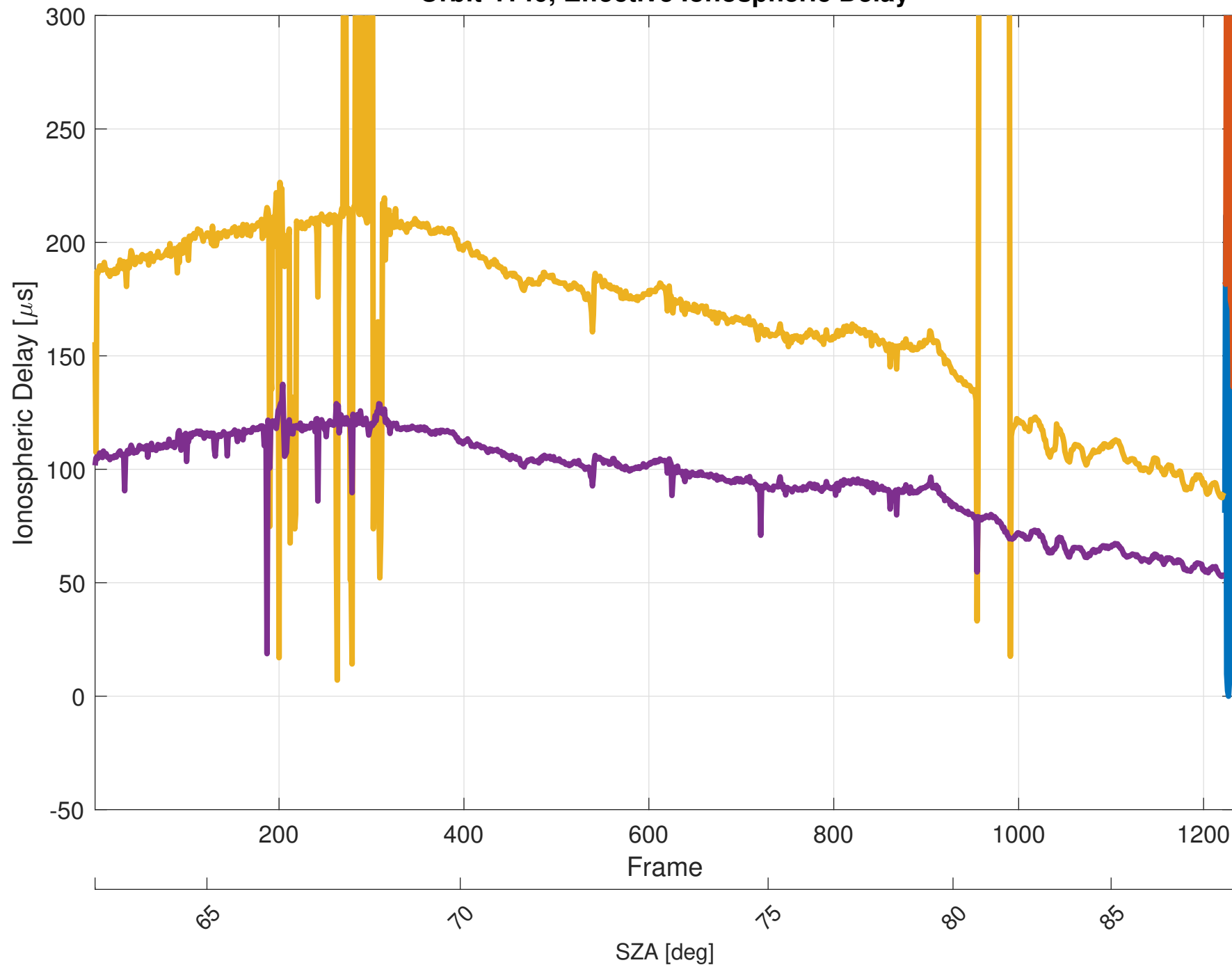
Orbit 4140, Effective Ionospheric Delay
